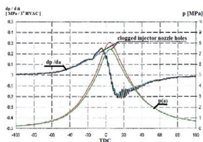
Fig. 3. The course of maximal speed of pressure escalation in the cylinder N0 of the 3 AL 25/30 engine with choked injector holes and the load of 220 kW in function of crankshaft rotation
