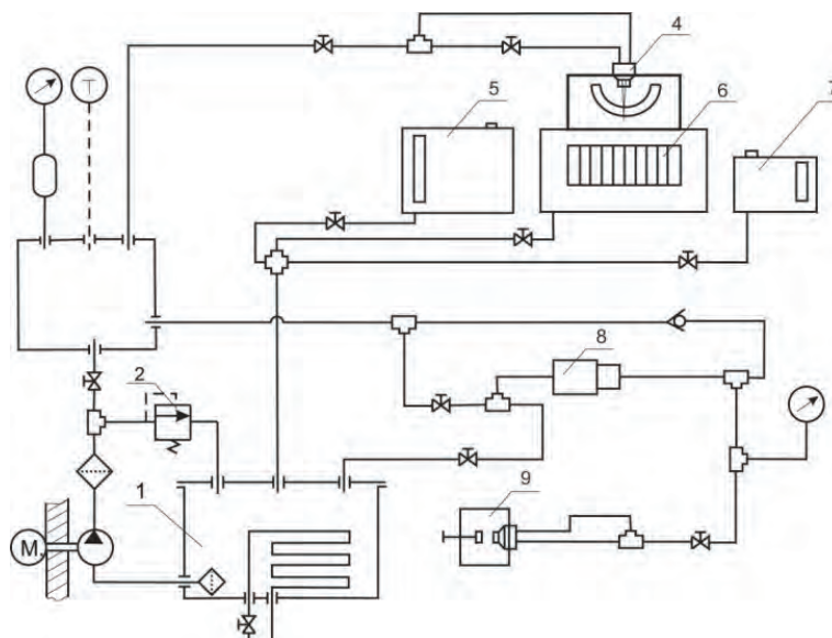
Fig.4. Ka - S/W station diagram: (1 – tank with radiator, 2 – safety valve, 3 – equalizing tank, 4 – tested injector, 5, 6, 7 – measuring vessels, 8 – pressure cylinder, 9 – injector grip to carry out leak proof test)
