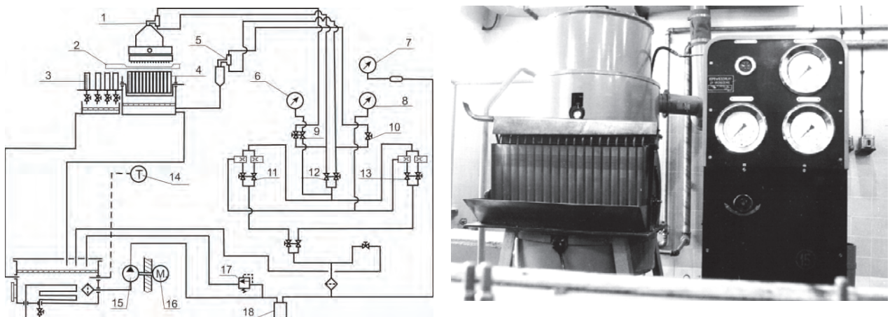
Fig.6. W-1762 type station diagram (1–tested injector, 2–drain pipe, 3–measuring vessels, 4–measuring tank, 5–standard sprayer, 6,7,8–manometers, 9,10,11,12,13–supply bus separating valves, 14–thermometers, 15–pump, 16–engine, 17–overflow valve, 18–equalizing tank)
