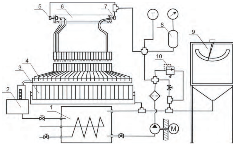
Fig.5. URS-97-R type station diagram (1–heat exchanger, 2,3–measuring tanks, 4–downpipe, 5–tested injector, 6–ring to install eighteen injectors, 7–startup injector, 8–cylinder, 9–measuring chamber, 10–safety valve)
