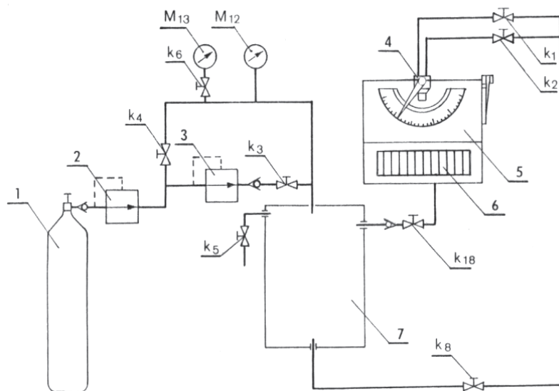
Fig. 2. Measurement station ITL WAT diagram (1 - compressed air cylinder, 2 - control valve, 3 - PU-7 valve, 4 - injector tested, 5 - measurement chamber, 6 - measurement chamber display window, 7 - fuel tank, k_5 - air bleed tank, k_1, k_2, k_3, k_4, k_6, k_8 and k_{18} - fuel supply pipes panel control valves, M12 i M13 - manometers)
