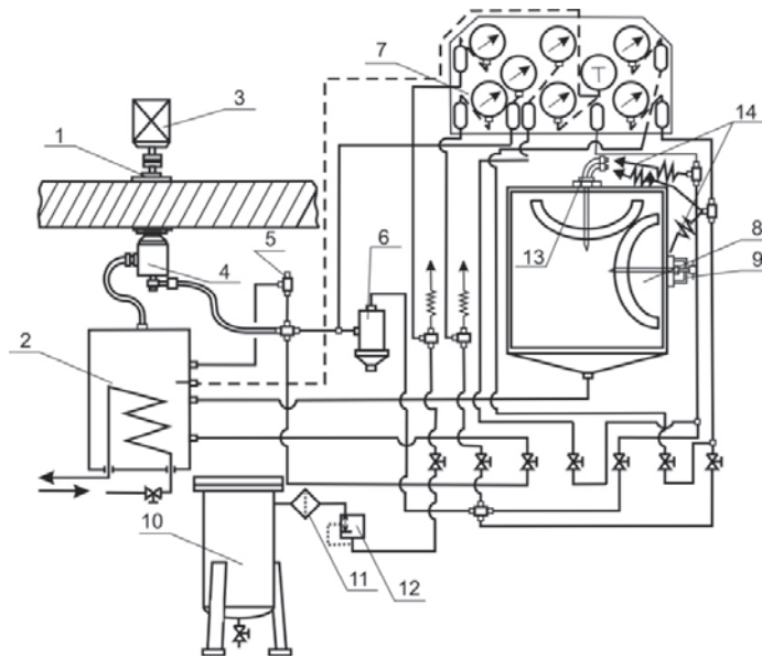
Fig 3. W - 1761 station diagram (1 – pump drive, 2 – fuel tank, 3 – electric engine, 4 – fuel pump, 5 – overflow valve, 6 – filter, 7 – measurement equipment panel, 8 – measurement chamber, 9 – side seating for fitting injectors, 10 – air dehumidifier, 11 – filter, 12 – reduction valve, 13 – injector tested, mounted in the upper seating, hoses linking the injector with the supply pipes)
