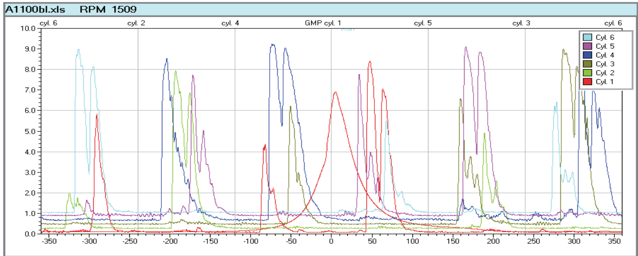
Fig. 7. Envelopes of vibration acceleration signals registered on one of the banks with six cylinders auxiliary diesel generator engine WOLA H12; engine speed = 1509 rpm, engine load = 100% of nominal load
