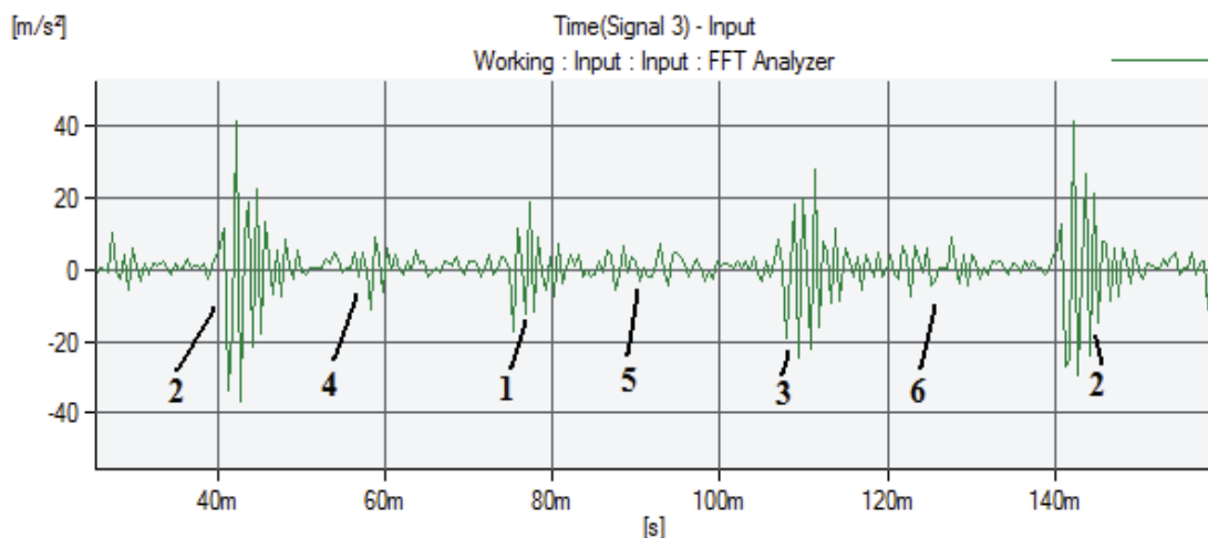
Fig. 2. Acceleration vibration signal measured on cylinder head number 2 in time domain. Engine firing order 1-5-3-6-2-4, plunger of the second section of fuel pump in normal operation
