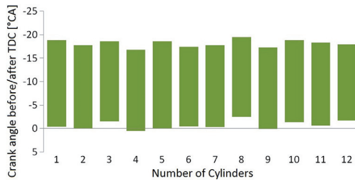
Fig. 8. Values of fuel injectors angles of opening and closing for auxiliary diesel-generator engine WOLA H12; engine speed = 1500 rpm, engine load = 100% nominal load
