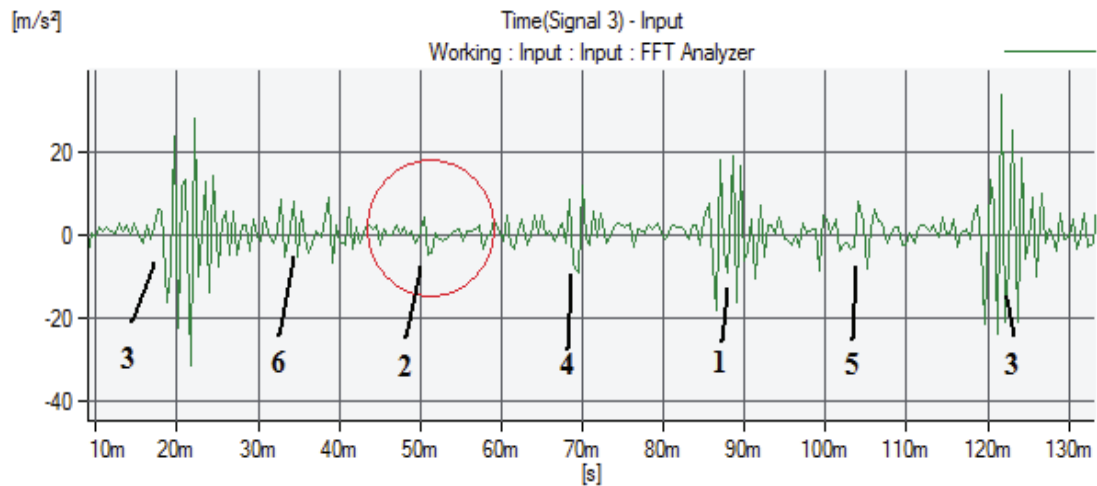
Fig. 1. Acceleration vibration signal measured on cylinder head number 2 in time domain. Engine firing order 1-5-3-6-2-4, plunger of the second section of fuel pump is blocked in upper position
