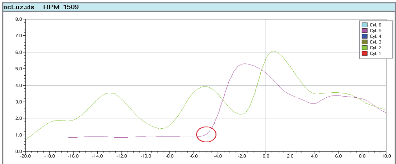
Fig. 6. Envelopes of vibration acceleration signals registered on the laboratory six cylinders diesel engine WOLA type 57H6Aa in „zoom“ mode circle – angle of fuel valves open; engine speed = 1509 rpm, engine load = 34 kW = 25% of nominal load
