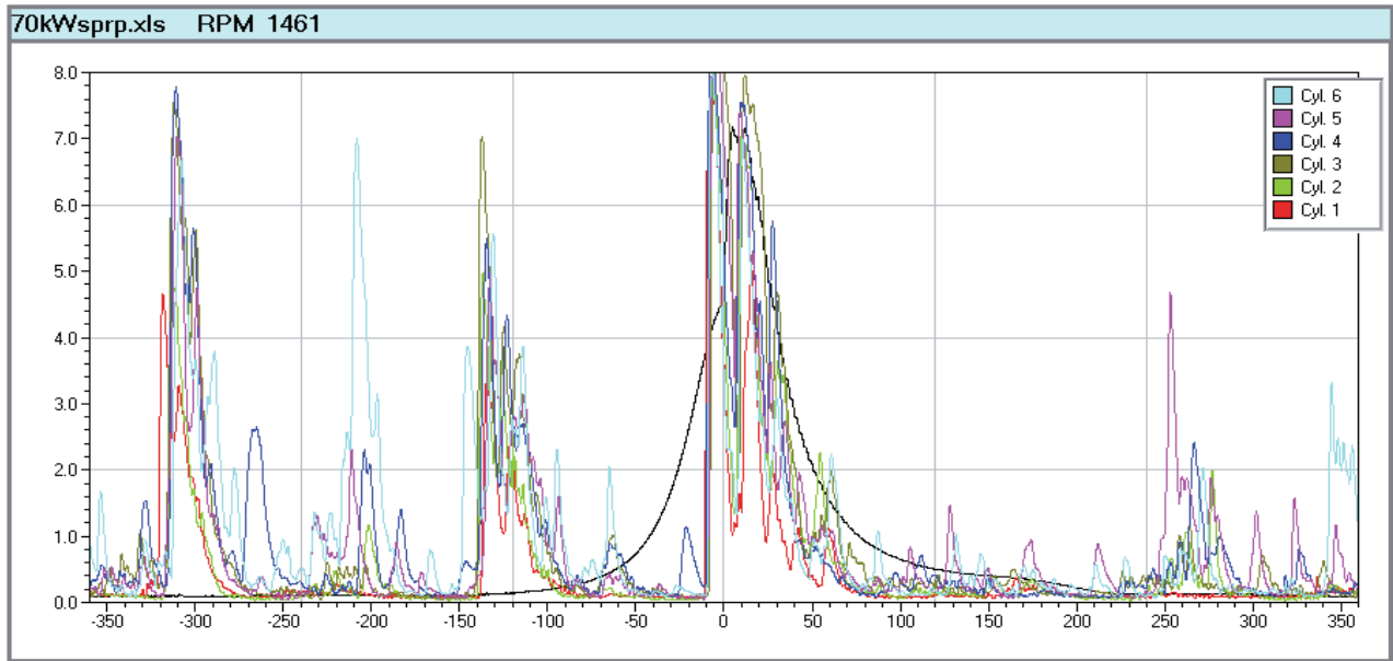
Fig. 3. Envelopes of vibration acceleration signals registered on the laboratory six cylinders diesel engine WOLA type 57H6Aa; engine speed = 1461 rpm, engine load = 70 kW = 50% of nominal load
