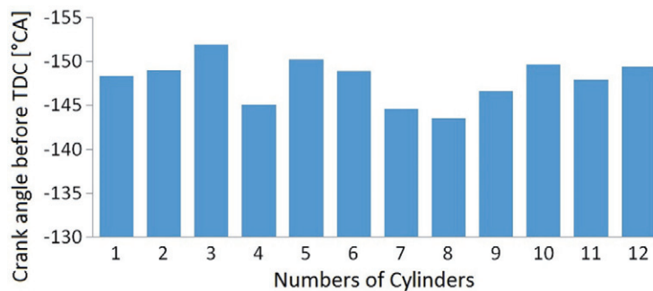
Fig. 9. Values of intake valves angles closing for auxiliary diesel-generator engine WOLA H12; engine speed = 1500 rpm, engine load = 100% of nominal load
