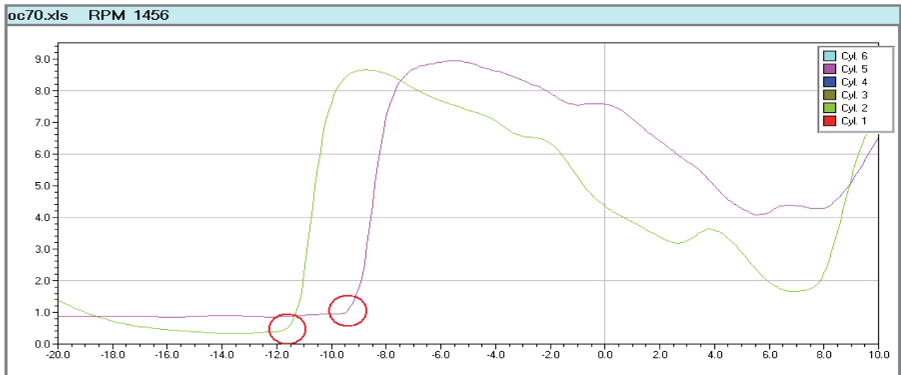
Fig. 5. Envelopes of vibration acceleration signals registered on the laboratory six cylinders diesel engine WOLA type 57H6Aa in „zoom“ mode circles – angles of fuel valves opens; engine speed = 1456 rpm, engine load = 34 kW = 25% of nominal load
