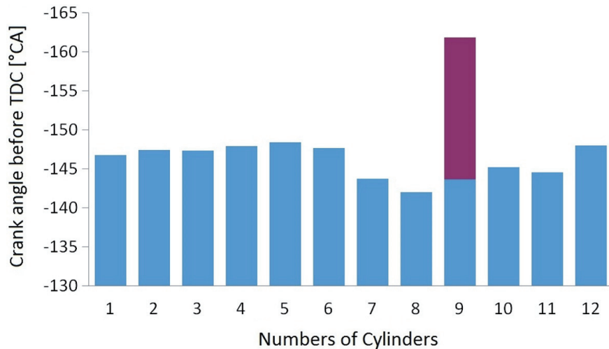
Fig. 10. Values of intake valves angles closing for auxiliary diesel-generator engine WOLA H12; engine speed = 1500 rpm, engine load = 100% of nominal load
