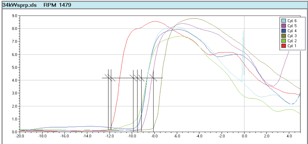
Fig. 4. Envelopes of vibration acceleration signals registered on the laboratory six cylinders diesel engine WOLA type 57H6Aa in „zoom“ mode – angles of fuel valves opens; engine speed = 1479 rpm, engine load = 34 kW = 25% of nominal load
