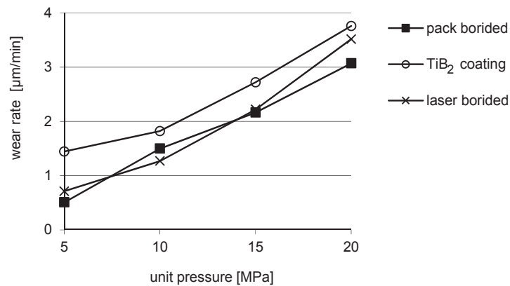
Fig. 5. Wear of counterpart with bearing alloy AlSn20 during cooperation with ring specimen (at 100 rpm)
