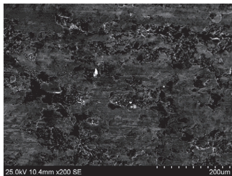
Fig. 6. SEM micrographs the pack borided surface layer and EDS analysis
