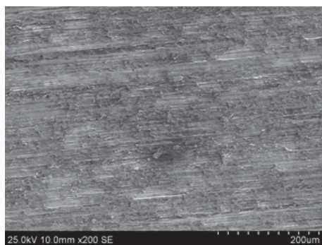
Fig. 7. SEM micrographs the TiB 2 coatings and EDS analysis
