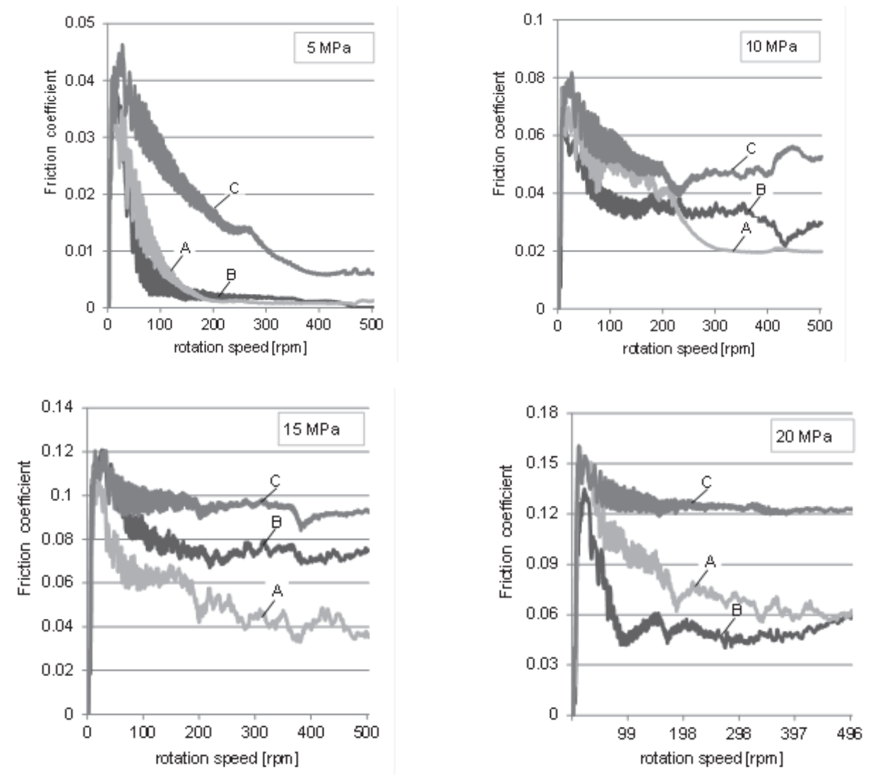
Fig. 2. Friction coefficient of ring specimens submitted to different surface treatment versus rotation speed: A – pack borided, B – coated \text{TiB}_2 , C – laser borided
