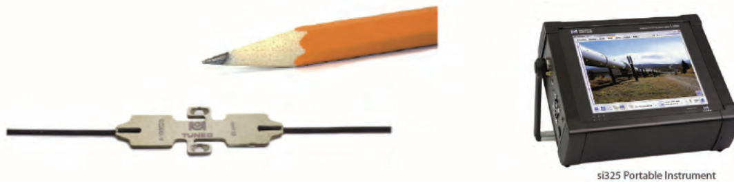
Fig. 3. Micron Optic FBG sensor and Micron Optic portable interrogator
