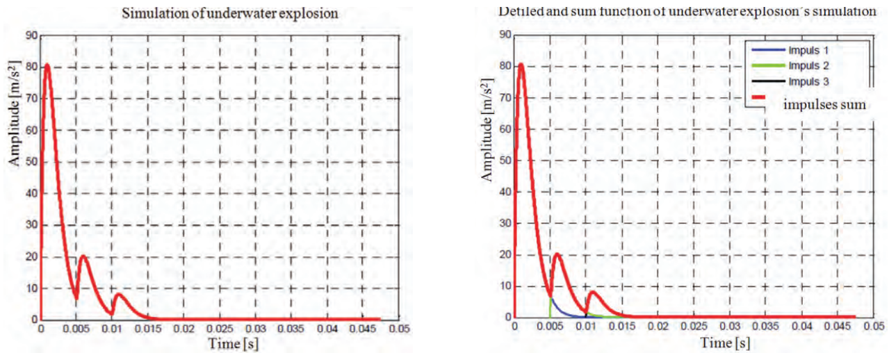
Fig. 1. Simulation of underwater explosion with three gas bubbles and assumed quotient of subsequent amplitude: A1/A2 = 0.25 and A1/A3 = 0.1 [10]
