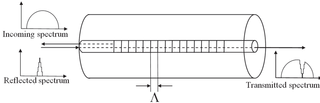
Fig. 2. Scheme of a FBG sensor with reflected and transmitted spectra
