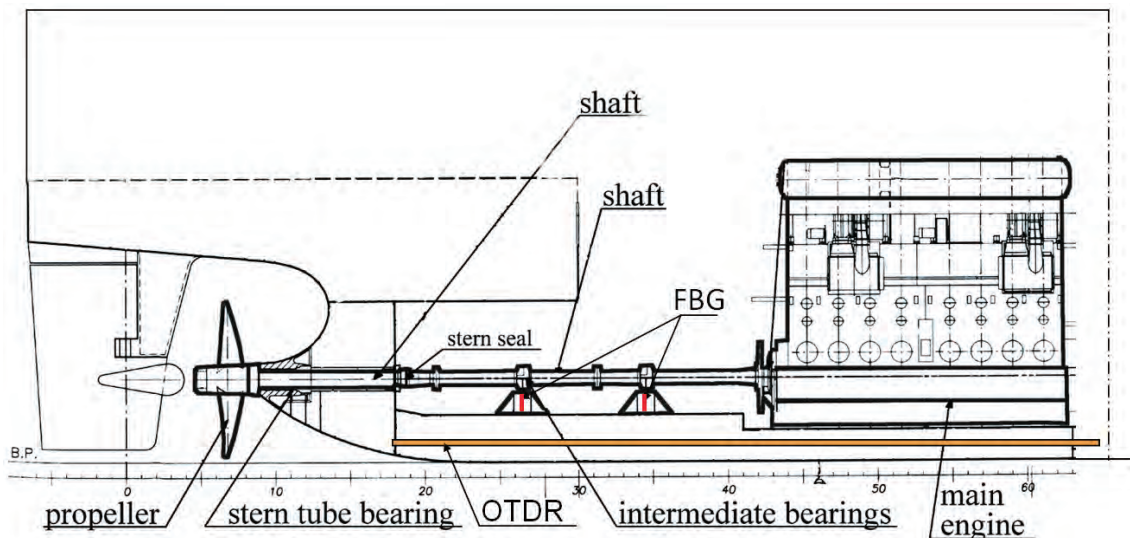
Fig. 5. Scheme of the sensors (OTDR and FBG) location on the ship
