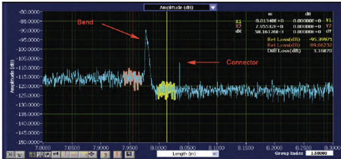
Fig. 4. Example signal from Luna optical backscatter reflectometer
