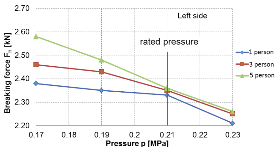
Fig. 4. Braking force change versus pressure in left (road side) wheel for different load
