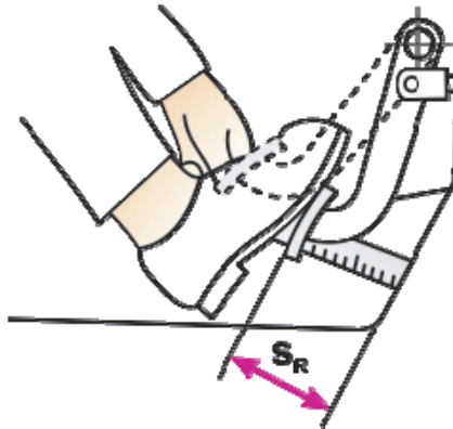
Fig. 3 Brake pedal reserve stroke measurement [3]
