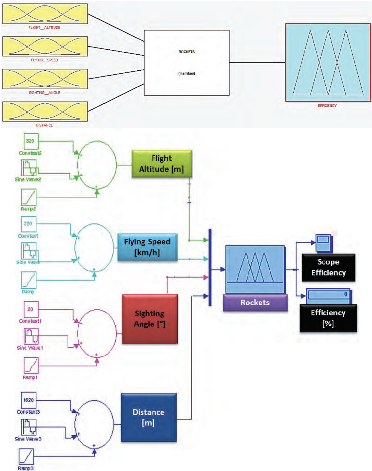
Fig. 2. Fuzzy efficiency estimation subsystem schematic diagram (Matlab Fuzzy Logic Toolbox and Simulink)
