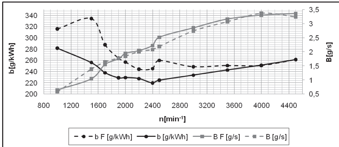
Fig. 4. Engine fuel consumption and engine specific fuel consumption curves with air filter being mounted and dismounted
