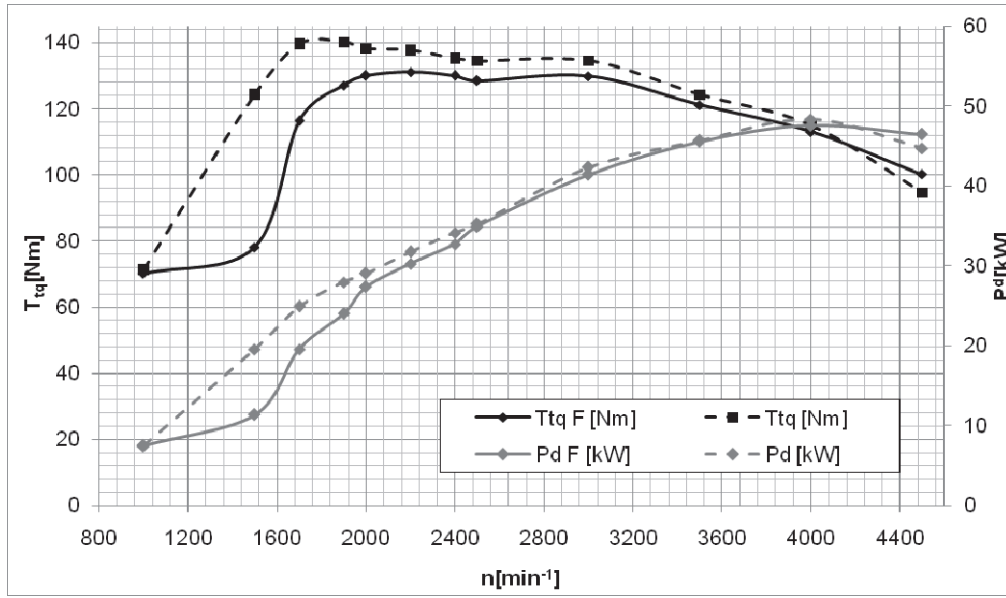
Fig. 3. Engine external characteristics with air filter being mounted and dismounted
