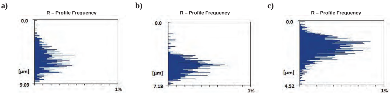
Fig. 6. The skewness for intermetallic coatings Ni_3Al for cutting inserts: a) square SNGA 120408 S01030A CB7015 ( R_{sk} = 0.407 \mu m ) and b) trigon WNMG 080408 S01030A CB7015 ( R_{sk} = 0.909 \mu m ) and c) trigon WNMG 080408 - KF with GC3215 ( R_{sk} = -0.423 \mu m )
