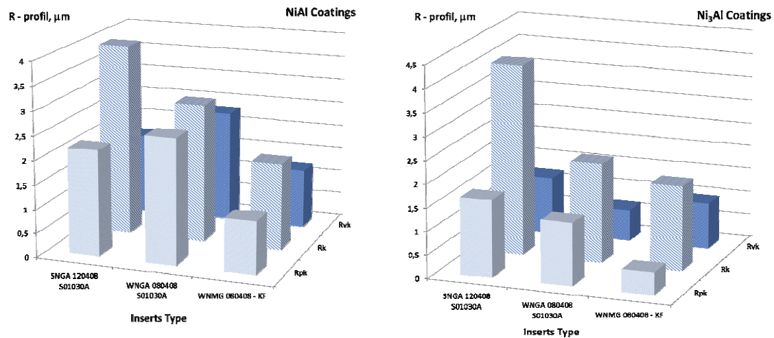
Fig. 2. The characterised parameters of the material ratio curve for intermetallic NiAl (left) and Ni 3 Al (right) coatings after – machining for selected inserts type
