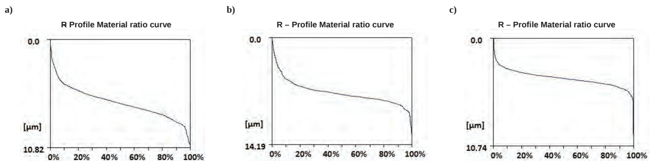
Fig. 3. The material ratio curve surface roughness intermetallic coatings NiAl for cutting inserts: a) square SNGA 120408 S01030A CB7015 ( R_a = 1.22 \mu\text{m} ) and b) trigon WNGA 080408 S01030A CB7015 ( R_a = 1.12 \mu\text{m} ) and c) trigon WNMG 080408 - KF GC3215 ( R_a = 0.61 \mu\text{m} )
