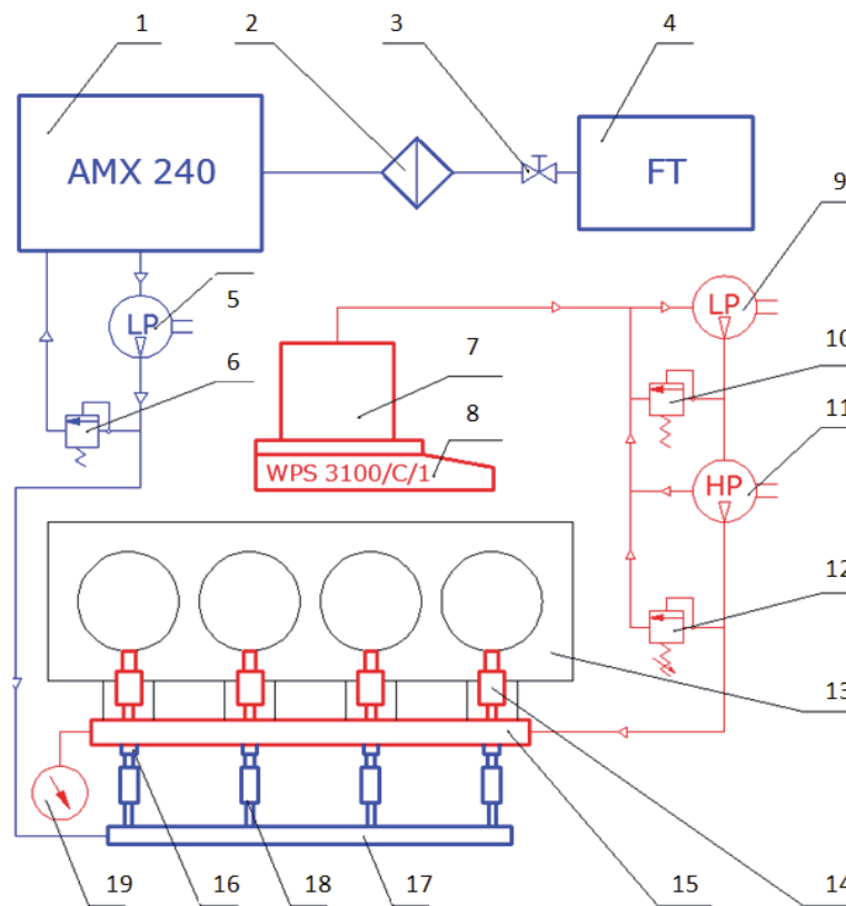
Fig. 2. System of power supply of testing engine (1 – grawimetric fuel's gauge, 2 – fuel's filter, 3 – cutting off valve, 4 – fuel's tank for system MPI, 5 – pomp of fuel of injection's petrol, 6 – controller of pressure of petrol's injection, 7 – fuel's tank for sytem of ignition dose, 8 – laboratory scales, 9 – powering pomp system of ignition dose, 10 – controller of low pressure of circuit of ignition dose, 11 – pomp of high pressure, 12 – pressure's controller of injection of ignition dose, 13 – testing engine, 14 – injection system of ignition dose, 15 – fuel splint of injection systems of ignition dose, 16 – approach duct, 17 – fuel slat of system MPI, 18 – injection system of petrol for system MPI, 19 – manometer pressure's of injection ignition dose)
