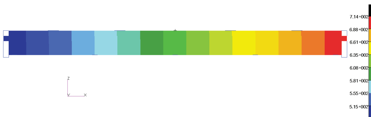
Fig. 6. Pontoons section immersion determined in numerical analysis
