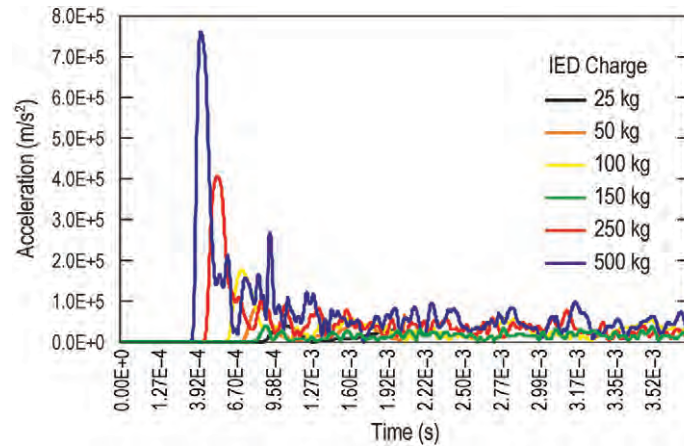
Fig. 9. Time history of the acceleration of selected node located on the side of the vehicle
