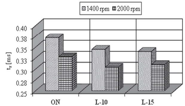
Fig. 5. Comparison of disintegration times of fuel streams t_r for the two engine speeds n=1400 rpm and n=2000 rpm
