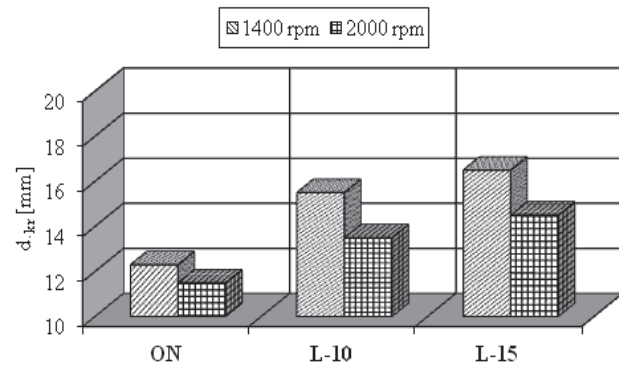
Fig. 4. Critical comparison of average droplet diameter d_{kr} for the rotational speed of the engine crankshaft n=1400 rpm and n=2000 rpm
