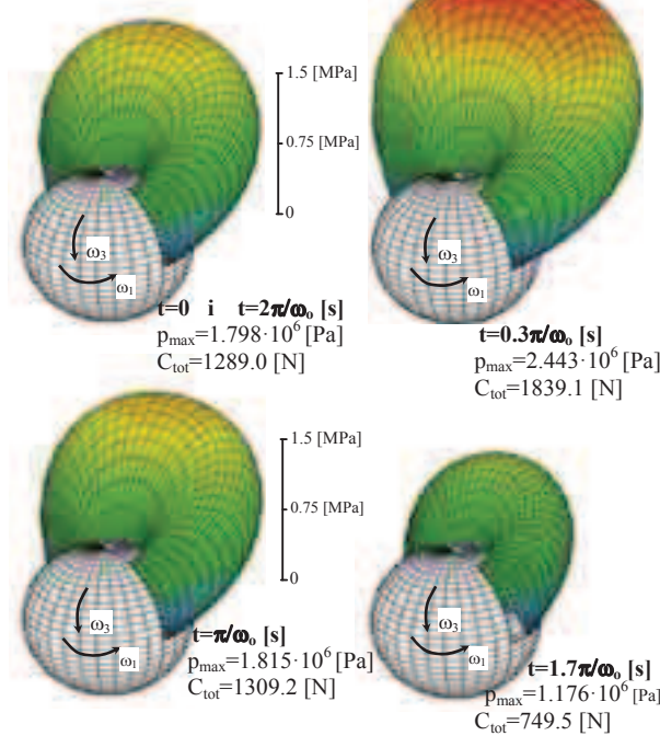
Fig. 1. The distributions of unknown function p presenting the solution of the partial differential and recurrence equation on the spherical surfaces restricting thin gap, and caused by the rotation of the spherical surface in circumferential direction \varphi and meridian direction \vartheta , simultaneously
