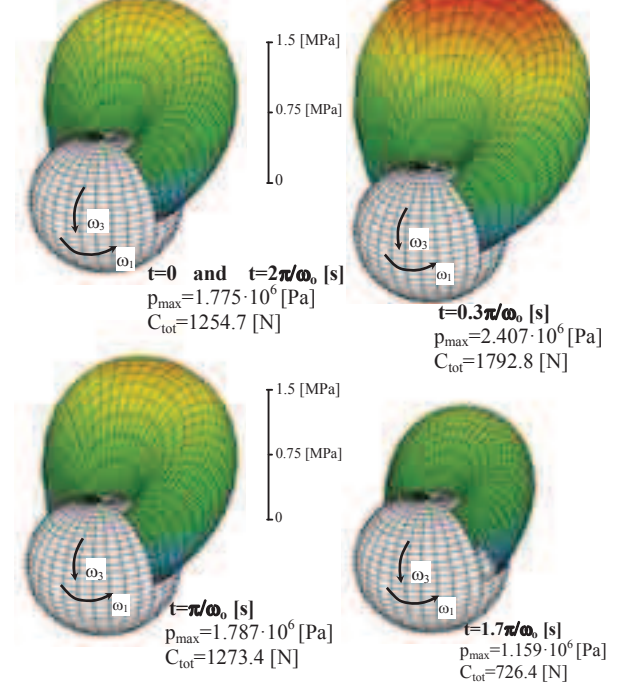
Fig. 2. The distributions of unknown function p (i.e. pressure) in gap, between two spherical surfaces caused by the rotation of the spherical surface in circumferential direction \varphi and meridian direction \vartheta , simultaneously. Magnetic effects are omitted i.e. M_i=0
