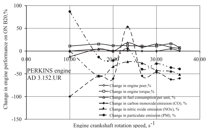
Fig. 3. Change in PERKINS AD.3.152.UR engine powered with diesel oil and biomix ON B20 of diesel oil (80%v/v) and a blend of butyl alcohol and rapeseed oil (20% v/v)
