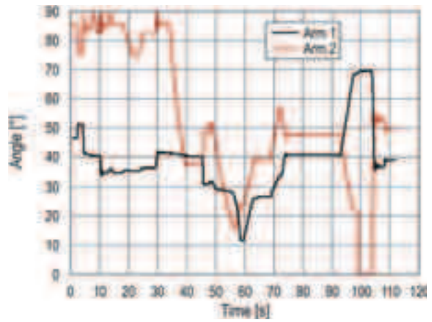
Fig. 7. Arm 1 and 2 angle to the vertical level versus time
