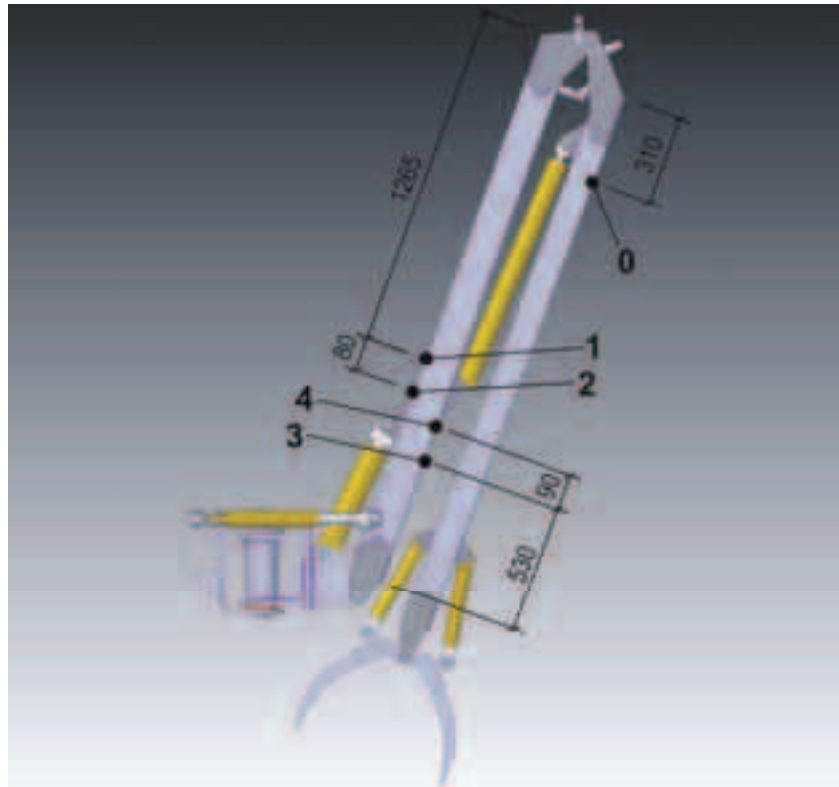
Fig. 3. Strain gauges placement
