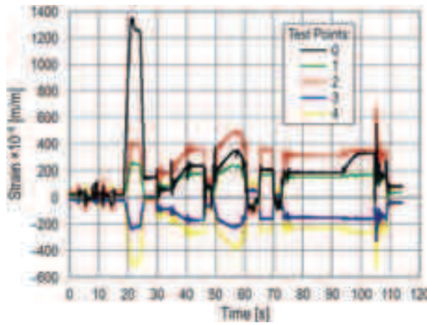
Fig. 6. Plots of the \varepsilon - t for test points 0–4
