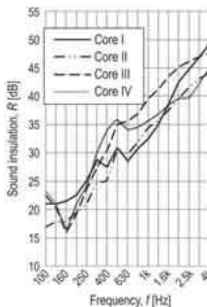
Fig. 11. Sound insulation coefficient
