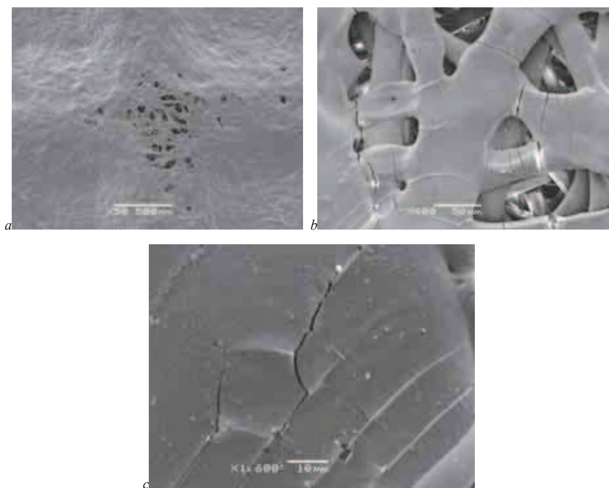
Fig. 9. a, b, c. SEM images of 4 (CuZnNi / NiCuFe / CuSn) sample surfaces
