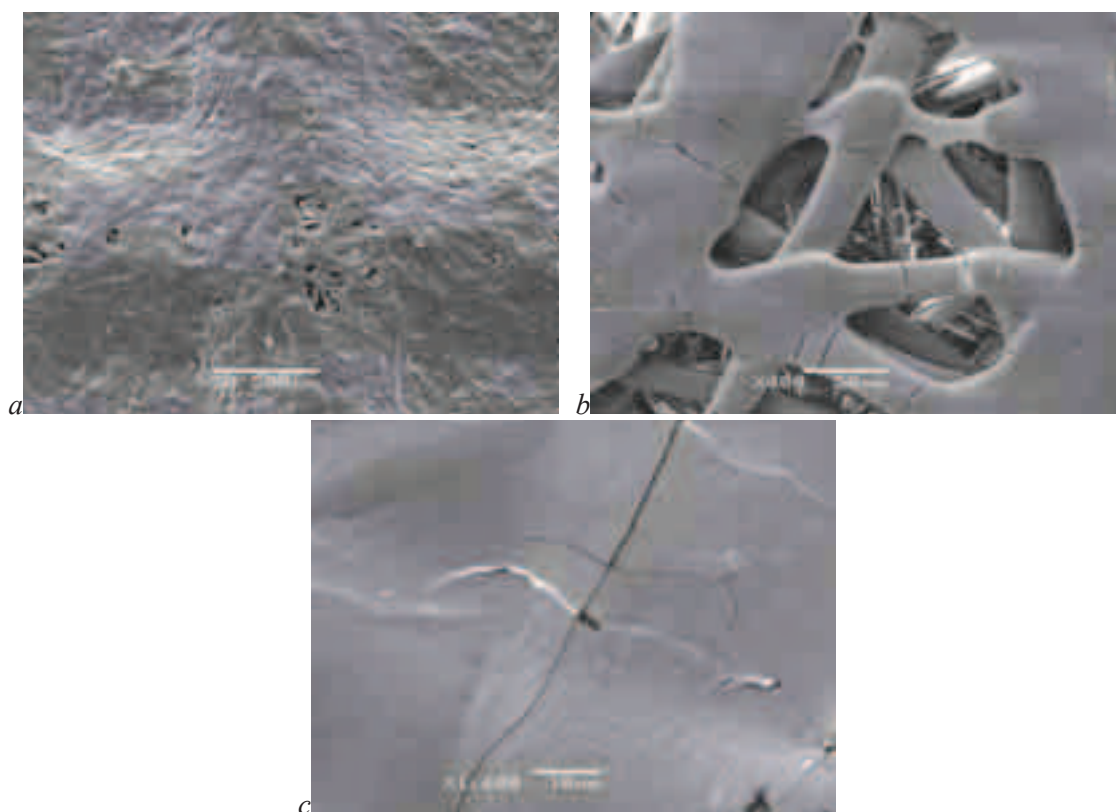
Fig. 7a, b, c. SEM images of 2 (NiCuFe) sample surfaces
