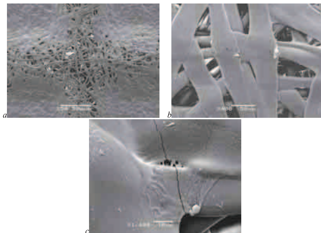
Fig. 8. a, b, c. SEM images of 3 (CuSn) sample surfaces
