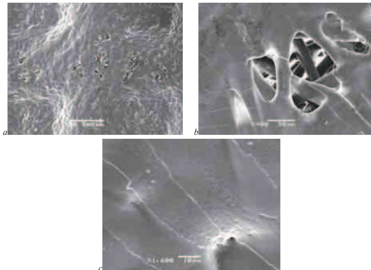
Fig. 6a, b, c. SEM images of 1 (CuZnNi) sample surfaces
