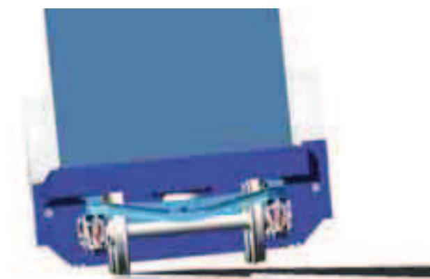
Fig. 14. Wagon moving at velocity of 120km/h on the arc of 250m radius with a view of detachment of wheels from the rails on the inner side of the arc
