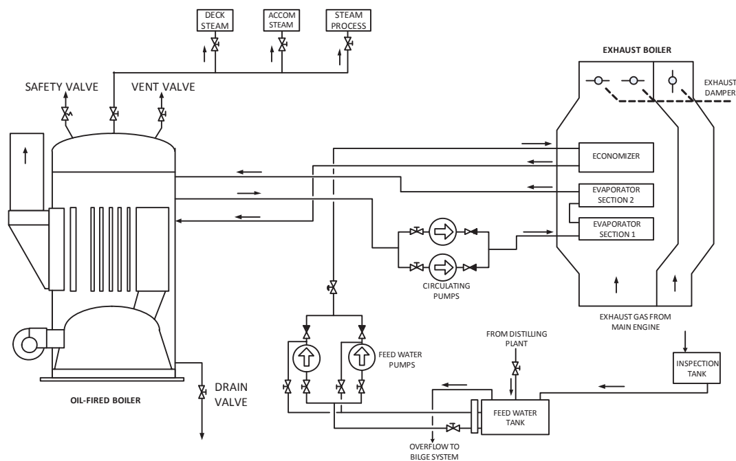
Fig. 1. The example of the steam system
