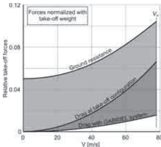
Fig. 5. Relative take-off forces for conventional aircraft and aircraft with GABRIEL system (shaded area shows difference) Fig. 6. Relative maximum take-off weight and static thrust
