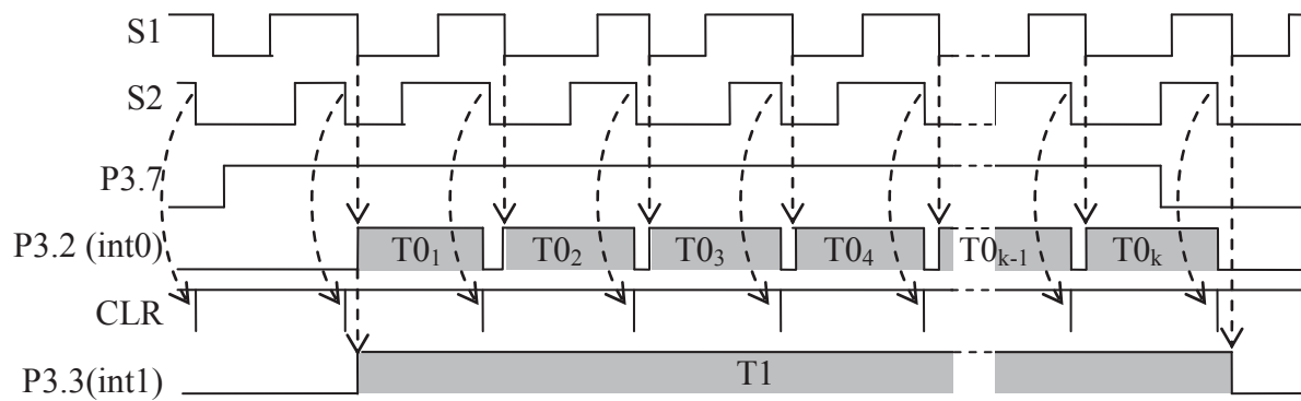
Fig. 2. Timing in the measuring system
