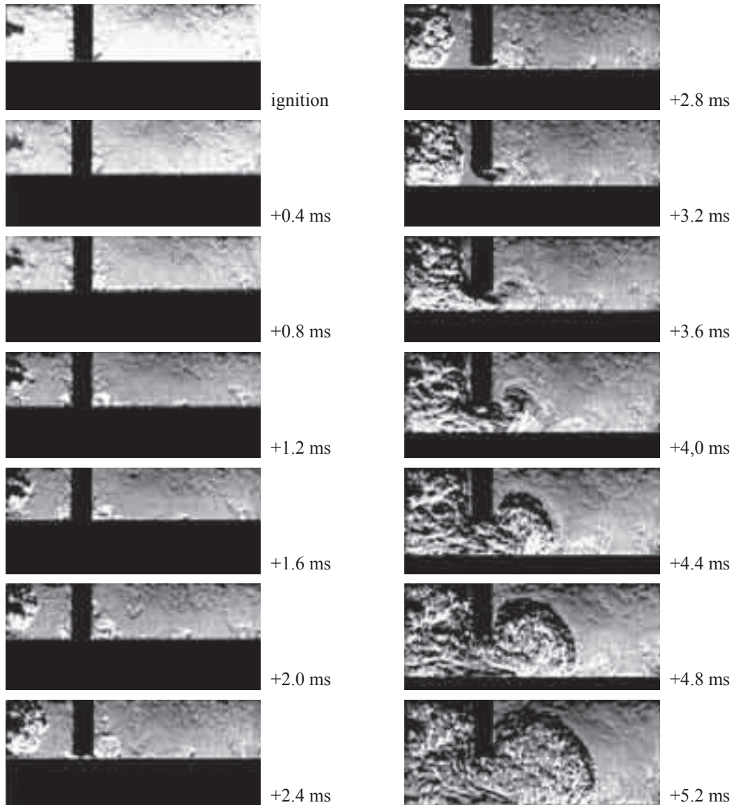
Fig. 16. Combustion process in a model combustion chamber during the tests using RCM: V_{kw} = 28\% , d = 3 \text{ mm} , ignition at the prechamber wall, \phi_{wz} = 10^\circ\text{CA BTDC}
