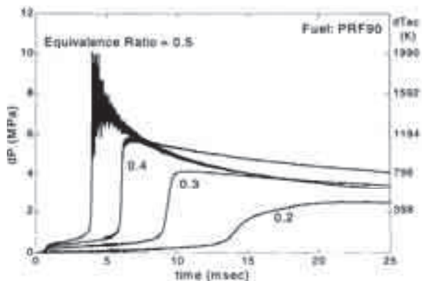
Fig. 12. Effect of equivalent ratio on ignition delay [4]
