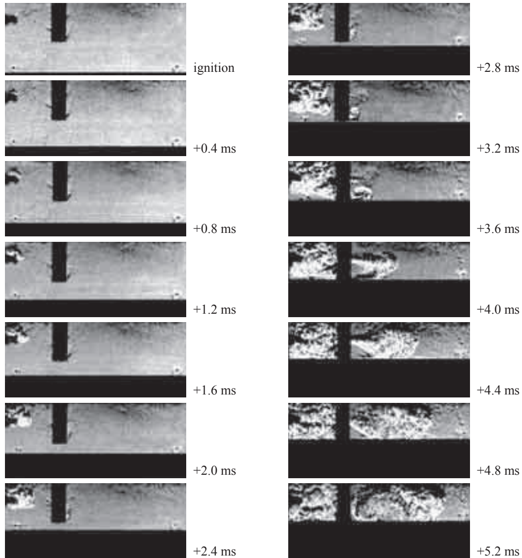
Fig. 17. Combustion process in a model combustion chamber during the tests using RCM: V_{kw} = 28\% , d = 3 mm, ignition at the prechamber wall, \phi_{wz} = 45^\circ\text{CA BTDC}
