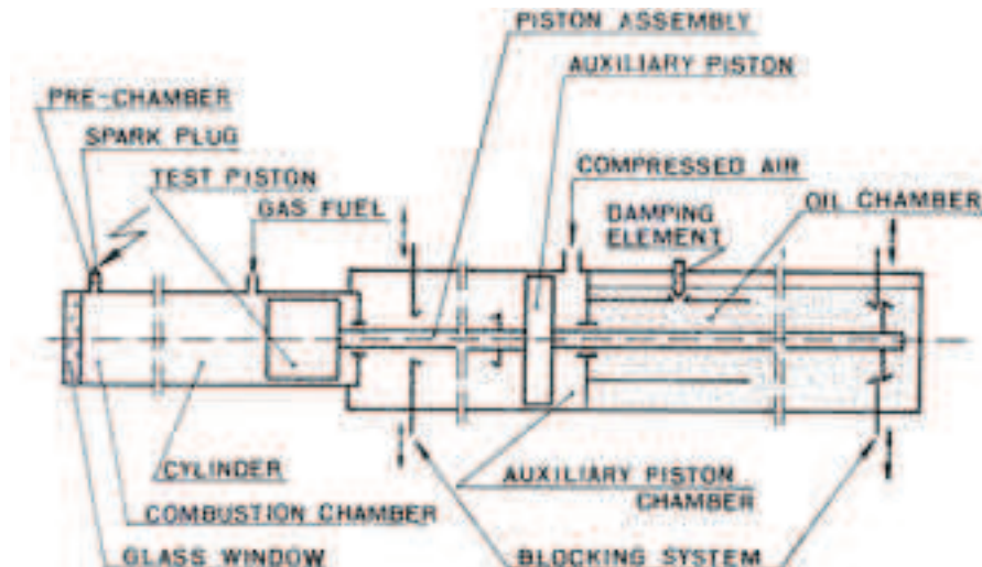
Fig. 1. Pneumatically driven RCM schema
