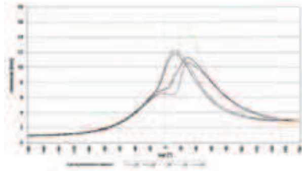
Fig. 4. The waveforms of pressure in the combustion chamber versus crankshaft rotation angle for different values of ignition advance angle
