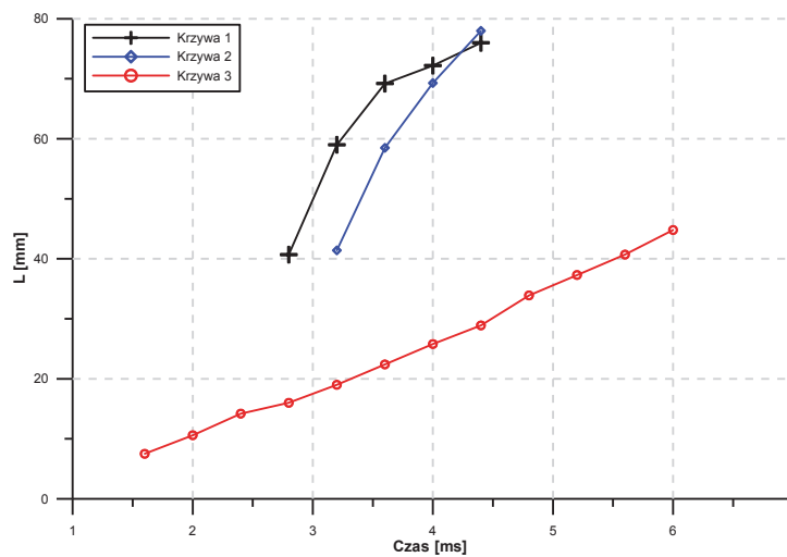
Fig. 7. The comparison of the stream front displacement for ignition advance angle 200 and 350 CA BTDC
