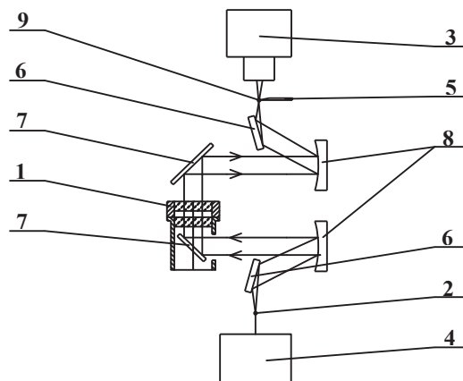
Fig. 3. Optical system, used in these experimental diagram: 1 - combustion chamber, 2, 9 - focus, 3 - drum camera, 4 - light source, 5 - optical knife, 6, 7 - plane mirrors, 8 - hemispherical mirror
