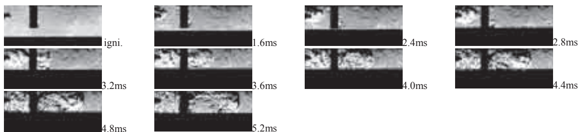
Fig.10. The combustion development in the new combustion system : ignition advance angle 35^{\circ} CA BTDC
