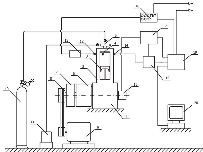
Fig. 2. Experimental set up schema. 1. Crank mechanism, 2. combustion chamber, 3. piston, 4. insert model combustion chamber, 5. refuelling and emptying system, 6. electromagnetic clutch, 7. flywheel, 8. external belt transmission, 9. electric motor, 10. pressurized bottle, 11. vacuum pump, 12. spark plug, 13. ignition apparatus, 14. piezoelectric transducer, 15. amplifier, 16. crank encoder, 17. indiskope 427, 18. ECU of optical system, 19. measurement card, 20. PC
