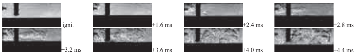
Fig. 5. The combustion development in the new combustion system: ignition advance angle 20^{\circ} CA BTDC
