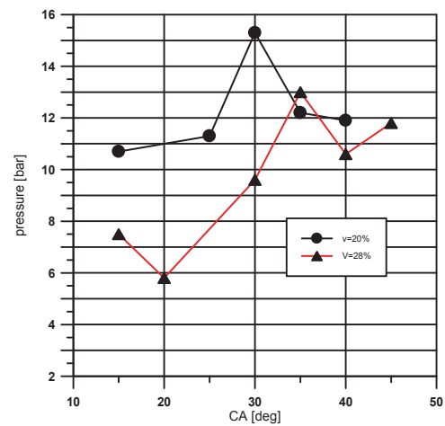
Fig. 12. The comparison of maximum cycle pressure as a function of ignition advance angle
