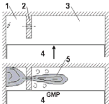
Fig. 1. Operating principle of the new combustion system: 1. Prechamber, 2. partition with orifice, 3. main combustion chamber, 4. piston, 5. stream of burned gases and radicals
