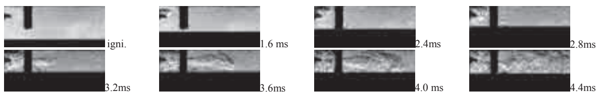
Fig. 6. The combustion development in the new combustion system : ignition advance angle 35^{\circ} CA BTDC
