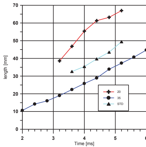
Fig. 11. Displacement flame front at the new combustion system and standard combustion system
