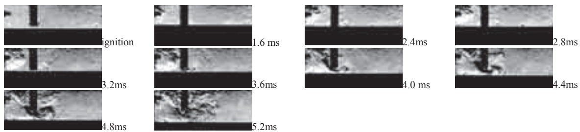
Fig. 9. The combustion development in the new combustion system : ignition advance angle 20^{\circ} CA BTDC
