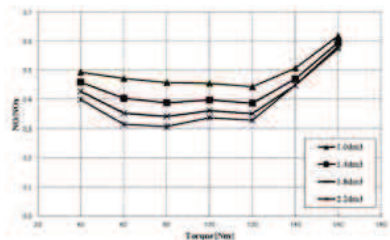
Fig. 5. The simulation computations concerning the influence of the change in the reactor solid volume at a cell packing density of 400 on the change of the content of NO in NO x
