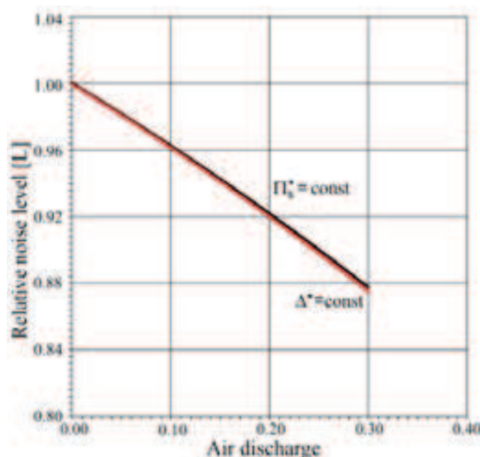
Fig. 4. Influence of air supply from behind the compressor to the place behind the turbine onto a relative level of engine noise depending upon the regulation method ( D = 0.3 m, r = 1 m)
