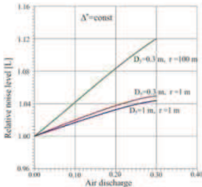
Fig. 7. Ratio of the levels of noise of the engines: one-flow engine equipped with the air discharge function to the environment and the “bypass” type of engine depending upon the amount of discharged air and the radius r as well as upon the diameter of the discharge nozzle D_5
