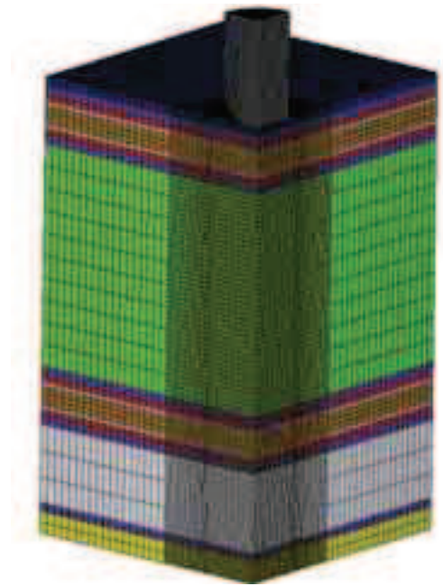
Fig. 2. The numerical model of the FSP–ALFC–PP system (an axonometric view)
