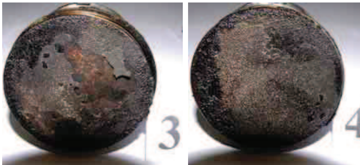
Fig. 8. View of the pistons after tests
