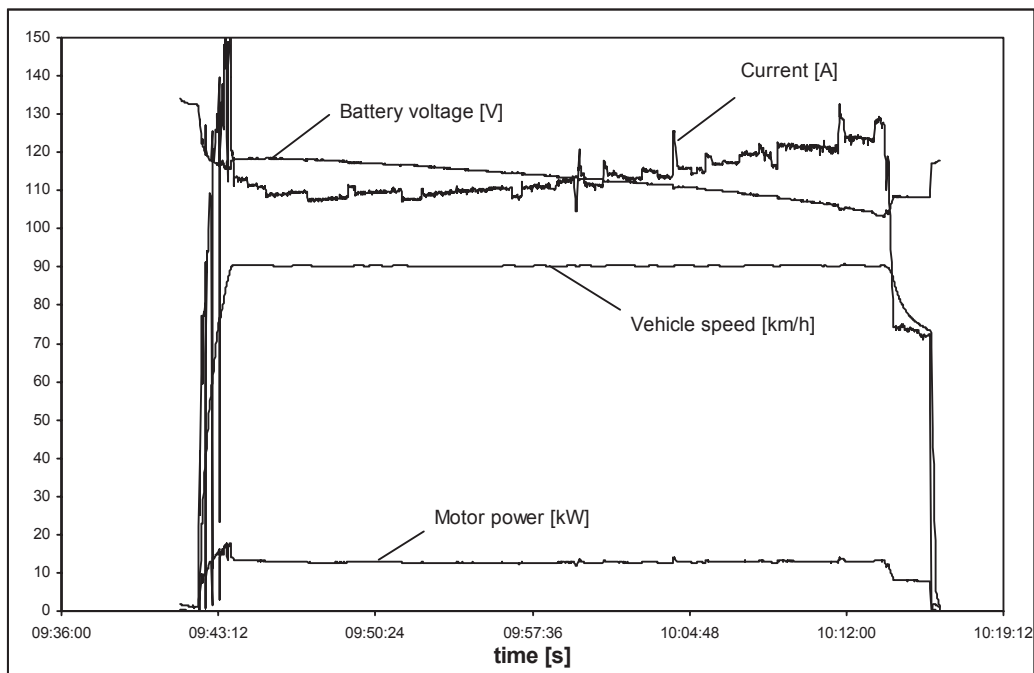
Fig. 6. The test at a speed of 90 km/h
