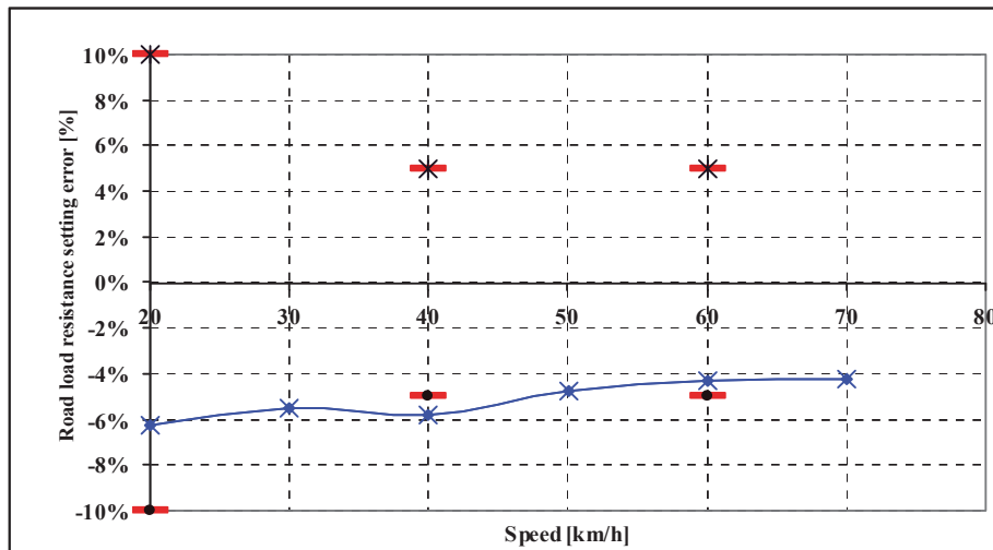
Fig. 3 The verification results of the total resistance
