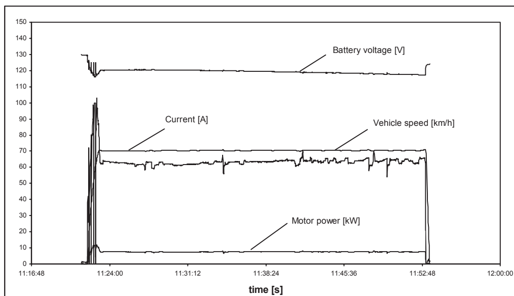
Fig. 5. The test at a speed of 70 km/h
