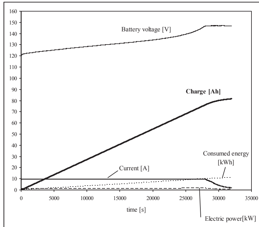
Fig. 13. Batteries charging measurements following the battery discharge, as in the records AR205_0_2011-01-26_16-00-41
