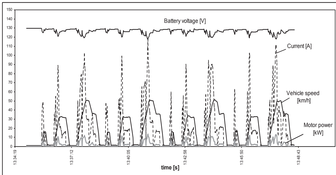
Fig. 11. The parameters of the selected NEDC test
