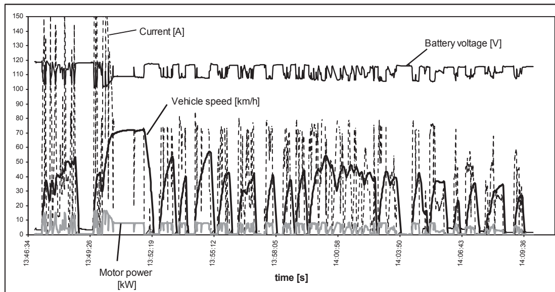
Fig. 9. FTP test parameters with a significant discharge of the vehicle battery. The record file AR205_0_2011-01-17_13-46-53
