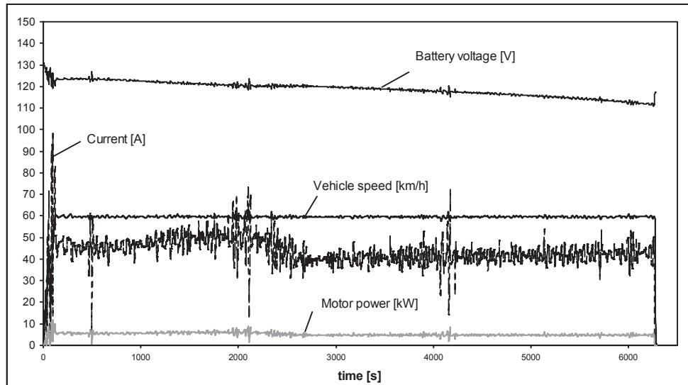
Fig. 12. The parameters of the selected test at 60 km/h, in accordance with the record AR205_0_2011-01-26_14-07-22
