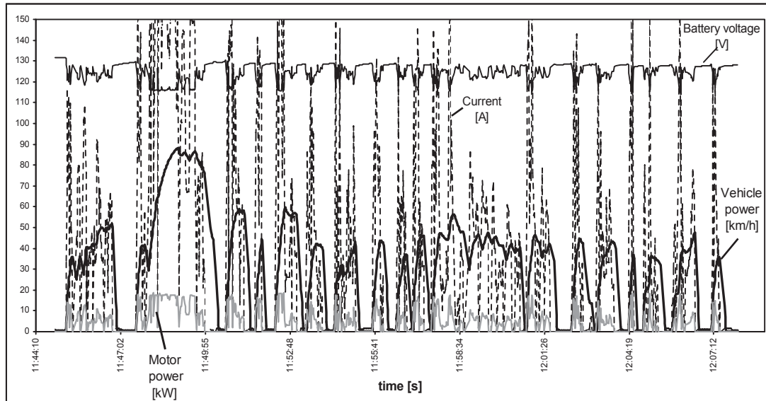
Fig. 8. FTP test parameters after charging the batteries. The record file AR205_0_2011-01-17_11-44-49
