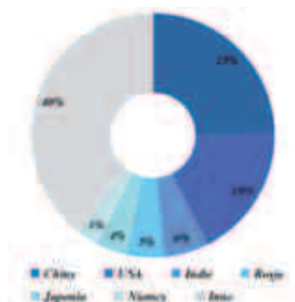
Fig. 2. \text{CO}_2 emissions by different countries [19]
