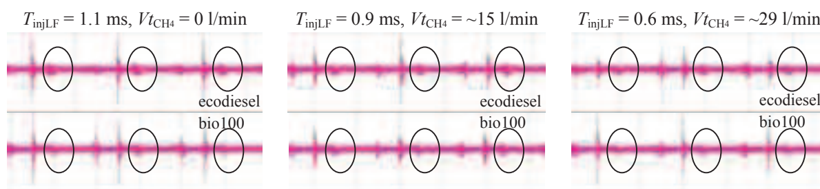
Fig. 4. Fragments of timing diagrams for vibration signals registered on the body of HATZ 1B40 engine for a set rotational speed of the crankshaft of 3000 rpm when the engine is fed with various air-fuel mixtures; marked oval fragments reflect the liquid fuel injection, its self-combustion and the onset of air-fuel mixture combustion
