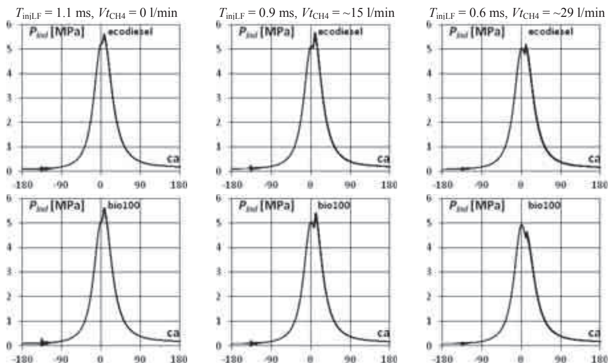
Fig. 2. Changes of pressure P_{ind} in the cylinder of the analysed engine fed with various air-fuel mixtures (20 fragments of engine performance cycles lining up)
