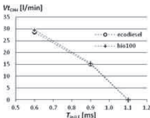
Fig. 1. Natural gas volumetric flow rate V_{tCH_4} which ensures steady engine performance at various doses (injection periods T_{injLF} ) of liquid fuels
