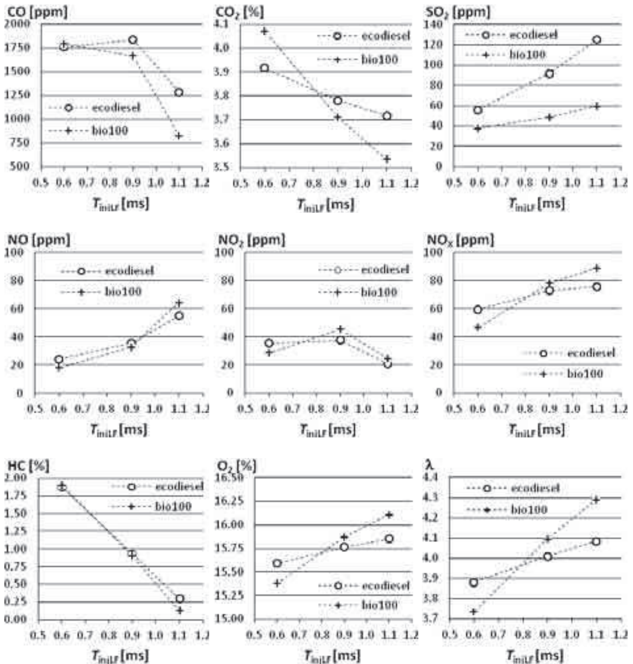
Fig. 3. Content of chosen substances in the exhaust gases of the analysed engine fed with various air-fuel mixtures (liquid fuel injection period T_{injLF} on the axes, volumetric flow rate of natural gas V_{tCH4} acc. to Fig. 1)
