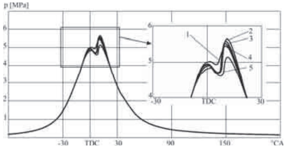
Fig. 1. Average changes of pressure in the combustion chamber at double-fuel engine fuelled with diesel oil (DO) at a varied constant angle of pilot dose injection of 20^{\circ}\text{CA} , at N_e=2\text{kW} , N=3000\text{ rpm} , and various shares of methane in the dose powering the engine: 1 – 100% DO, 2 – 50% DO+CNG, 3 – 33% DO+CNG, 4 – 22% DO+CNG, 5 – 12% DO + CNG
