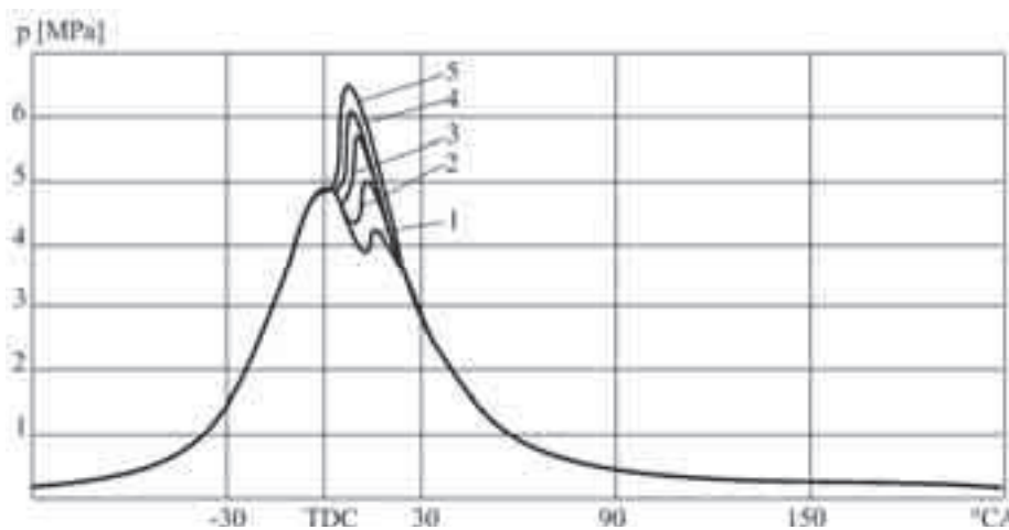
Fig. 2. Average changes of pressure in the combustion chamber at dual fuel engine supply with diesel oil at varied pilot dose injection angle, at N_e=2\text{k} , N=3000\text{ rpm} , a dose of diesel oil of 22%: 1 – 16^{\circ}\text{CA} , 2 – 18^{\circ}\text{CA} , 3 – 20^{\circ}\text{CA} , 4 – 22^{\circ}\text{CA} , 5 – 24^{\circ}\text{CA}
