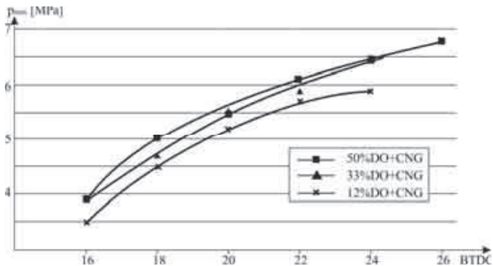
Fig. 3. The effects of advance angle of the pilot dose injection on the maximum pressure of combustion, at various proportions of diesel oil and CNG
