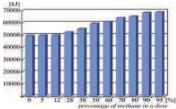
Fig. 4. Power demand of a dual-fuel self-ignition engine supplied with a mixture of methane and diesel oil
