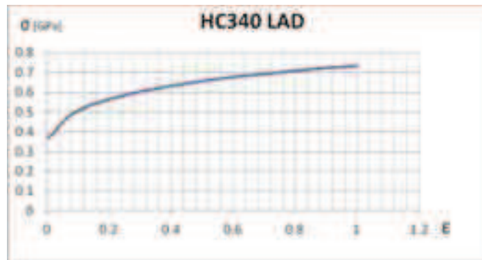
Fig. 4. Hardening curve for HC340 LAD g_0 = 2\text{ mm}
