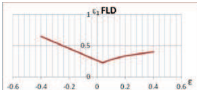
Fig. 5 Forming Limit Diagram for HC340 LAD with g_0 = 2\text{ mm} [10]
