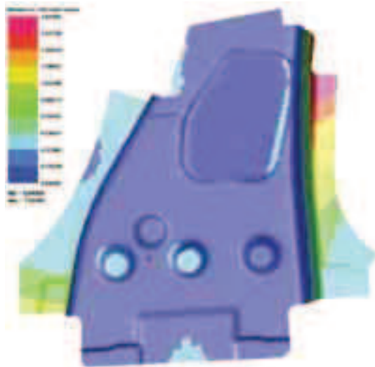
Fig. 9. Compensated part without full chain optimization
