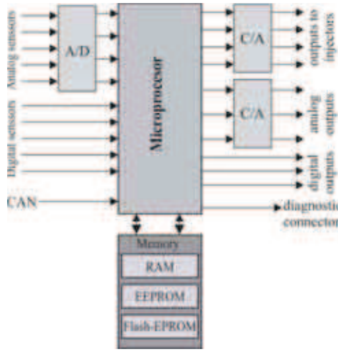
Fig. 1. A diesel engine's controller - a sketch of architecture
