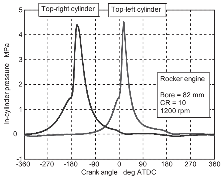
Fig. 5. Modelled combustion pressure in the 2-cylinder rocker engine
