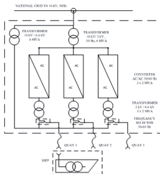
Fig. 3. The “Shore To Ship” concept for ferry terminals
