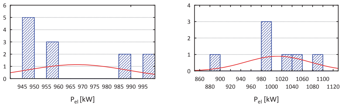
Fig. 8. Electric load histogram while berthing in the port; Świnoujście (left diagram) and Ystad (right diagram)
