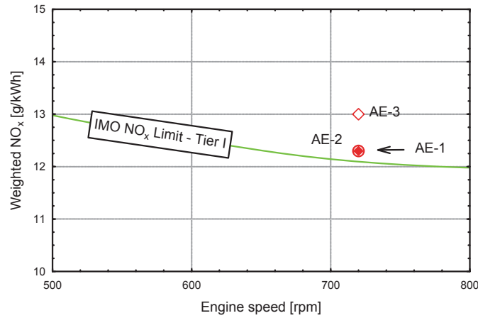
Fig. 7. NOx emission factors for ship diesel engine generators in Tier I limit
