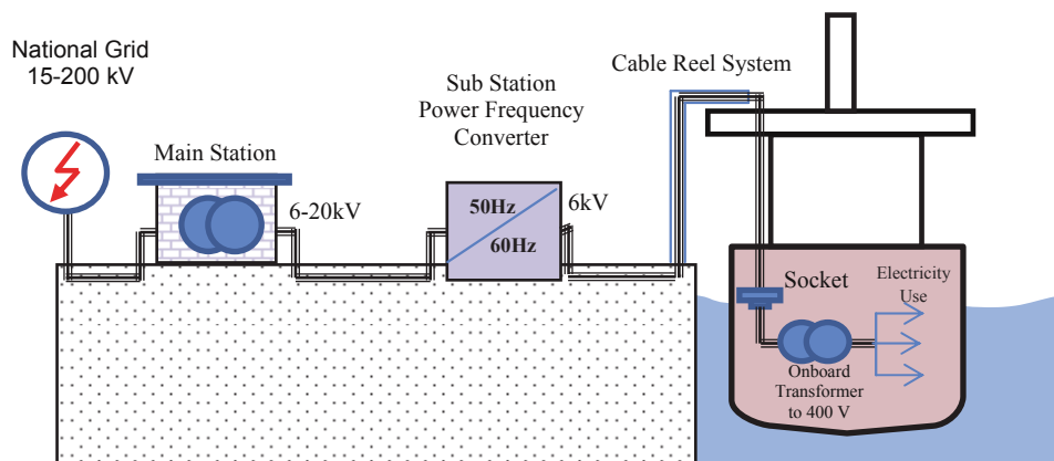
Fig. 2. The scheme of vessel electric supply system configuration in the port according to EU regulations
