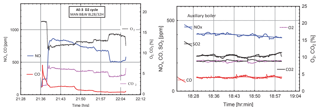
Fig. 6. The exemplary, registered exhaust gas composition for engine AE 3 and heating boiler
