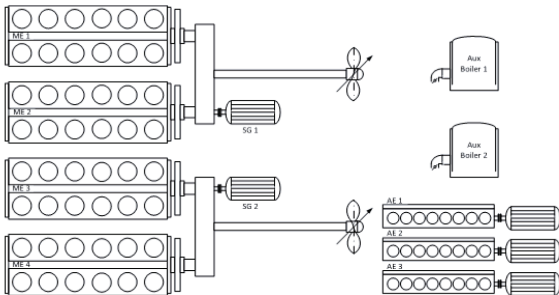
Fig. 4. The scheme of configuration for the main and auxiliary propulsion of m/f Skania
