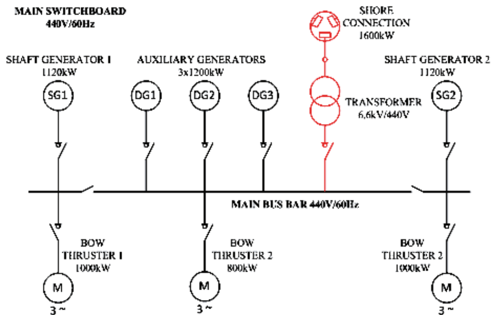
Fig. 5. The configuration of the electric supply system with the planned shore connection (in red)
