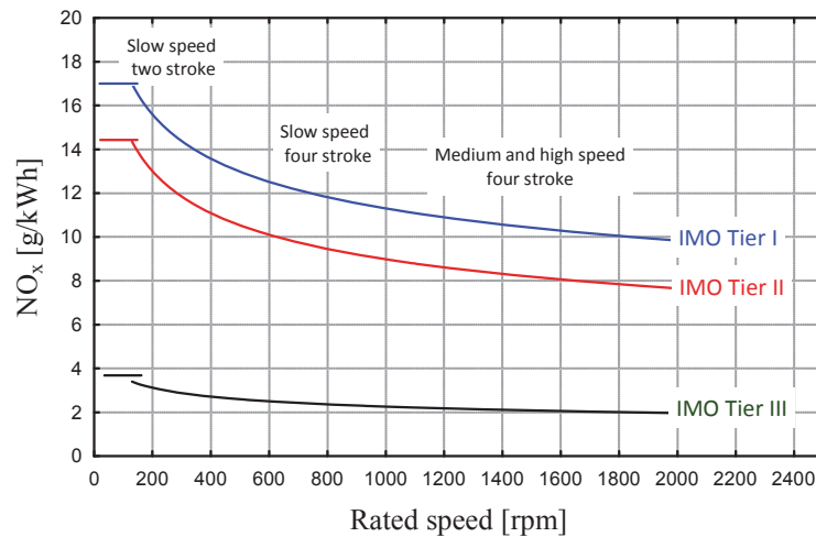
Fig. 1. Nitrogen oxides emission limits for marine engines
