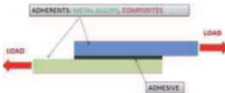
Fig. 2. Adhesive joint
