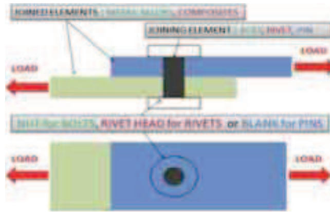
Fig. 1. Mechanical joint
