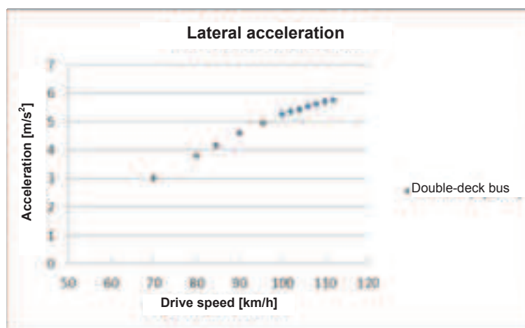
Fig. 6.2. Extreme values of the lateral acceleration measured at the centre of mass
