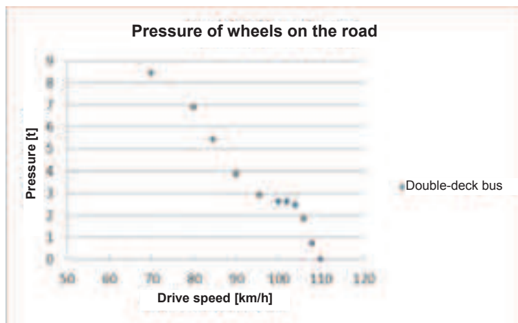
Fig. 6.3. Minimum values of the sum of the pressures of wheels on the road on one bus side
