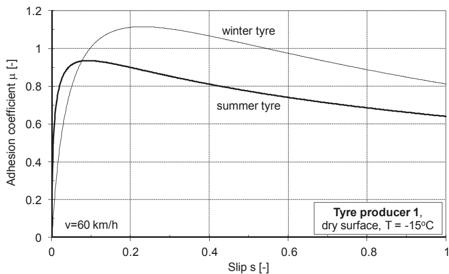
Fig. 9. Adhesion characteristics \mu(s) for summer and winter tyres – negative temperatures
