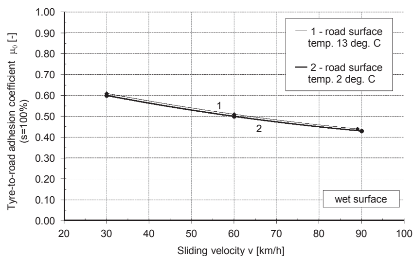
Fig.5. Velocity characteristics \mu_0(v) for different ambient temperatures
