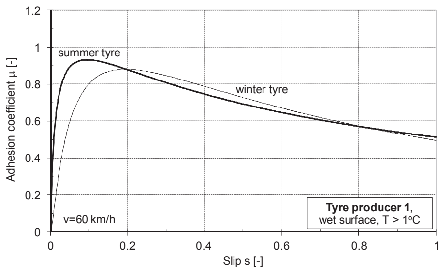
Fig. 7. Adhesion characteristics \mu(s) for summer and winter tyres – positive temperatures
