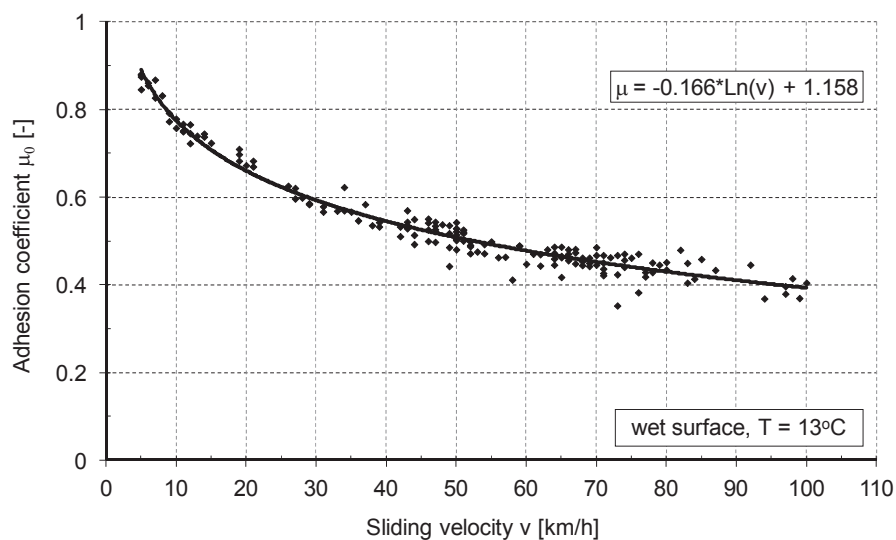
Fig. 4. Example of velocity characteristic \mu_0(v)
