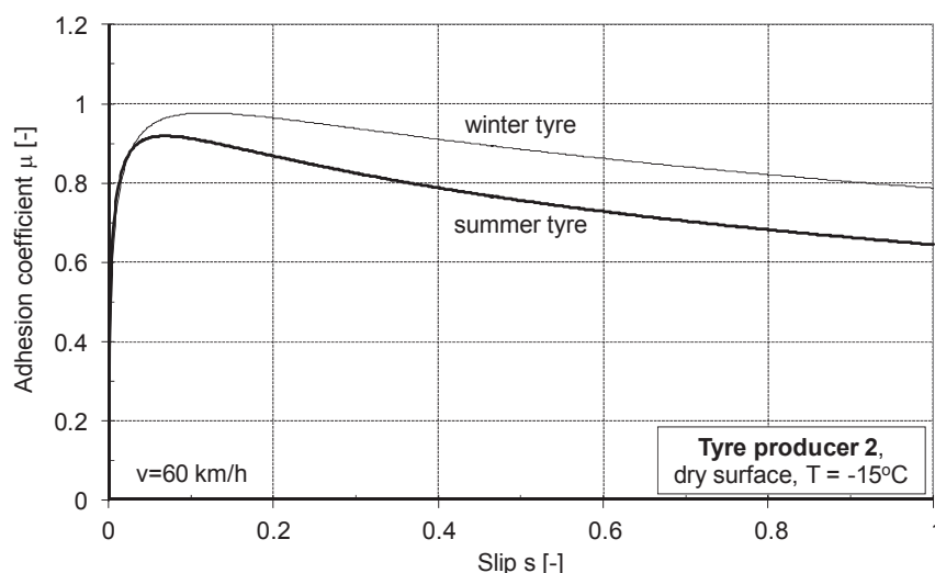
Fig. 10. Adhesion characteristics \mu(s) for summer and winter tyres – negative temperatures
