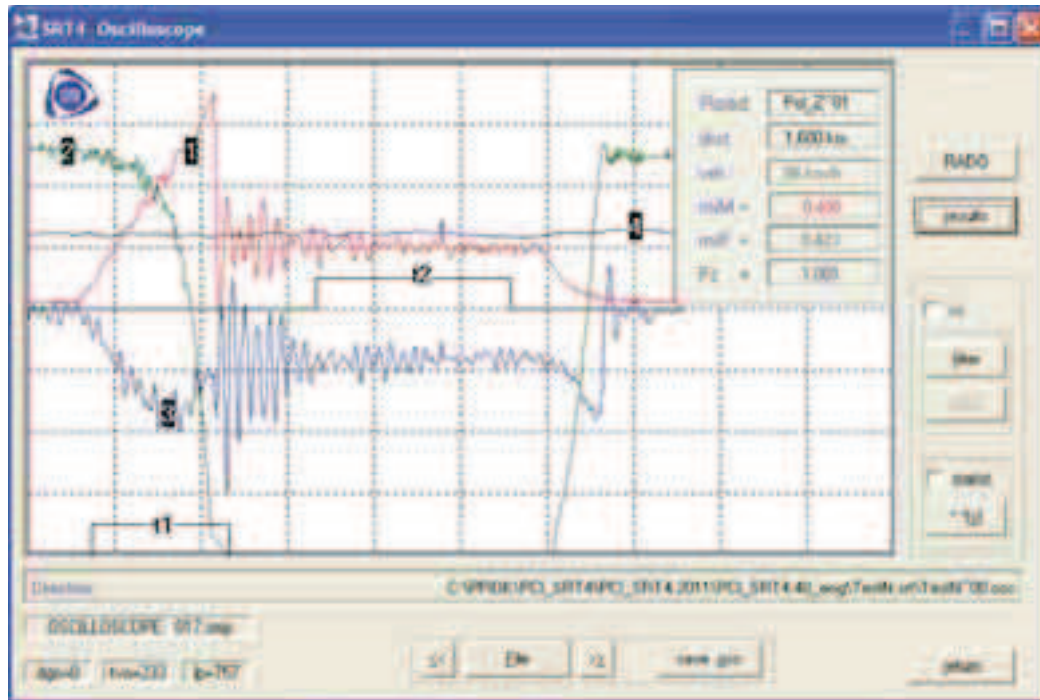
Fig. 3. Measurement signals of dynamometer trailer: 1-wheel velocity, 2-braking torque, 3-wheel friction force, 4-wheel normal load
