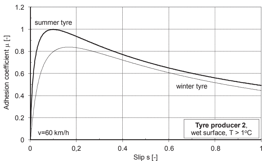
Fig. 8. Adhesion characteristics \mu(s) for summer and winter tyres – positive temperatures
