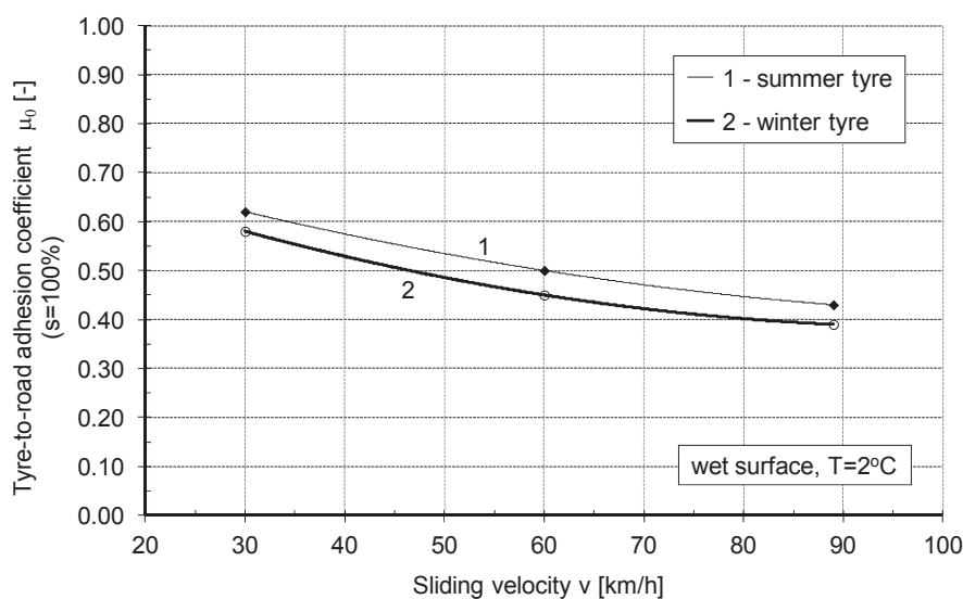
Fig.6. Comparison of summer and winter tyres
