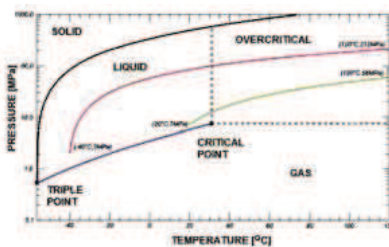
Fig. 4. Isochoric process of heated CO 2 (density of 1120 and 809kg/m 3 )
