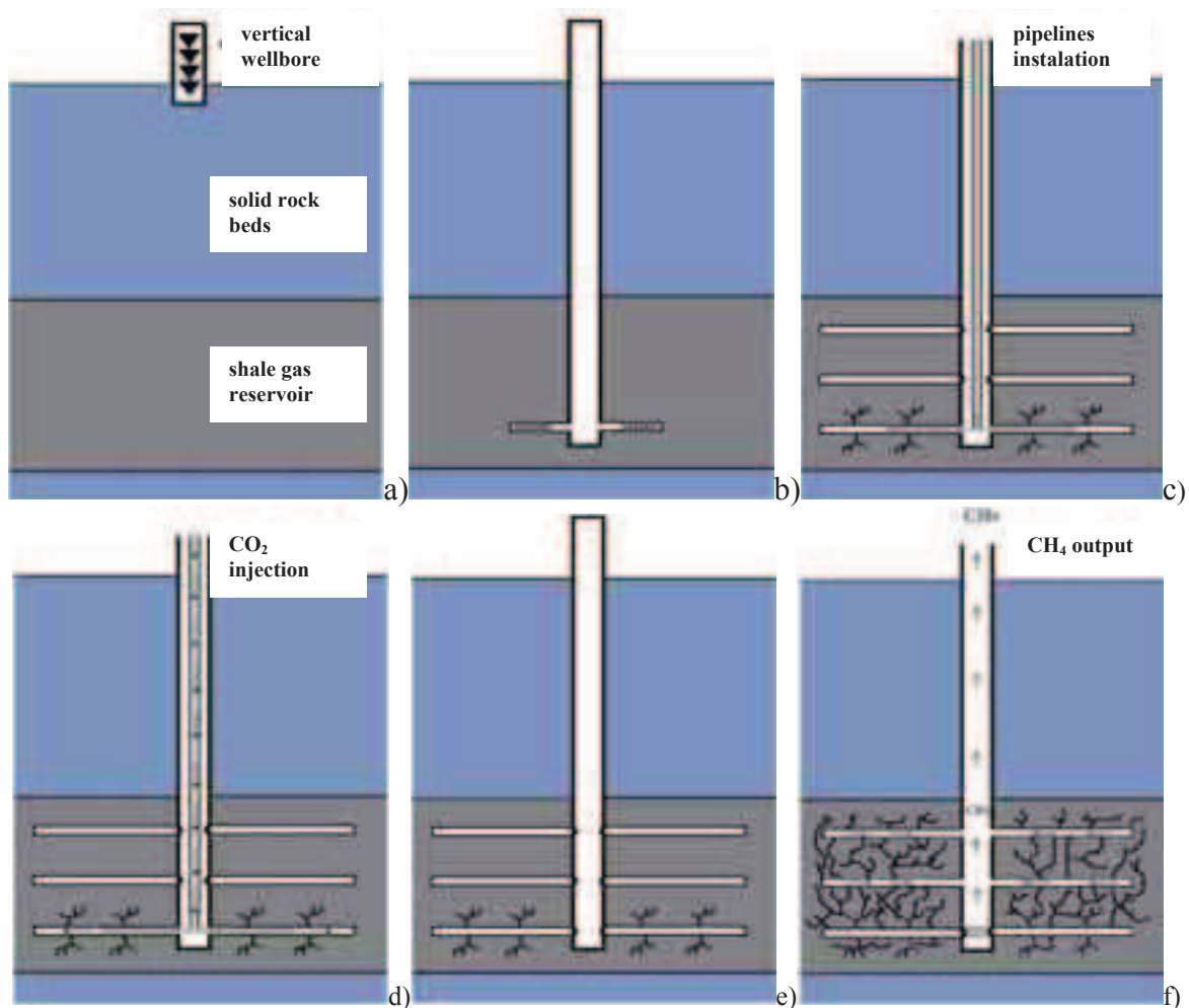
Fig. 3. Scheme of method of gas shale fracturing and gas recovery coupled with carbon dioxide storage
