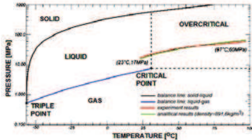
Fig. 6. Comparison of analytical and experimental tests of CO 2 heating
