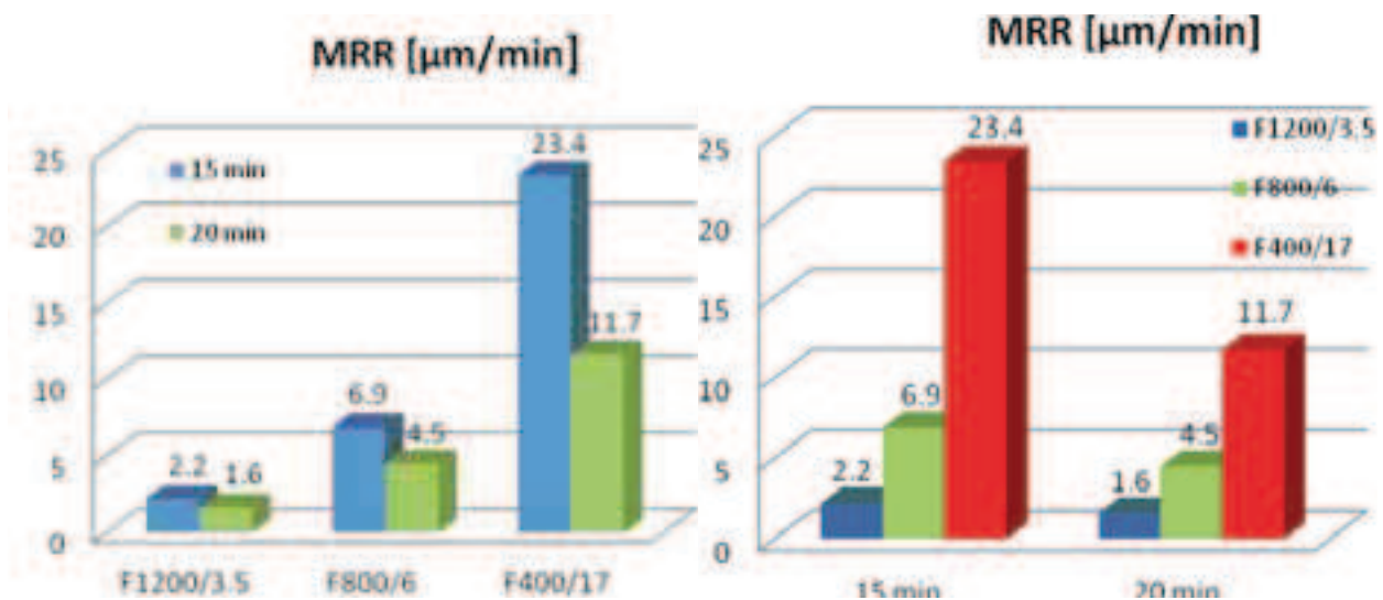
Fig. 6. Test results of MRR in \mu\text{m}/\text{min} depending on grains size and lapping time
