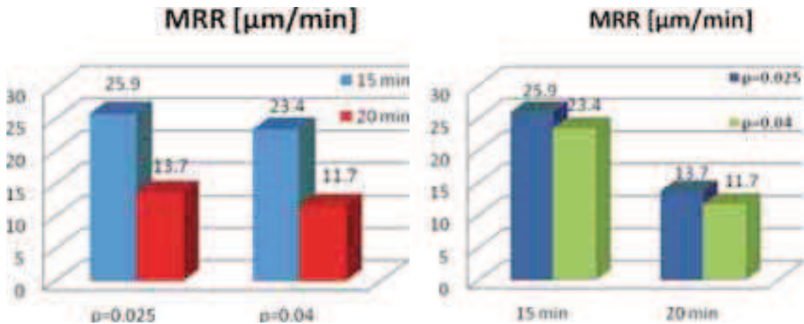
Fig. 9. Test results of MRR in \mu m/min depending on lapping pressure
