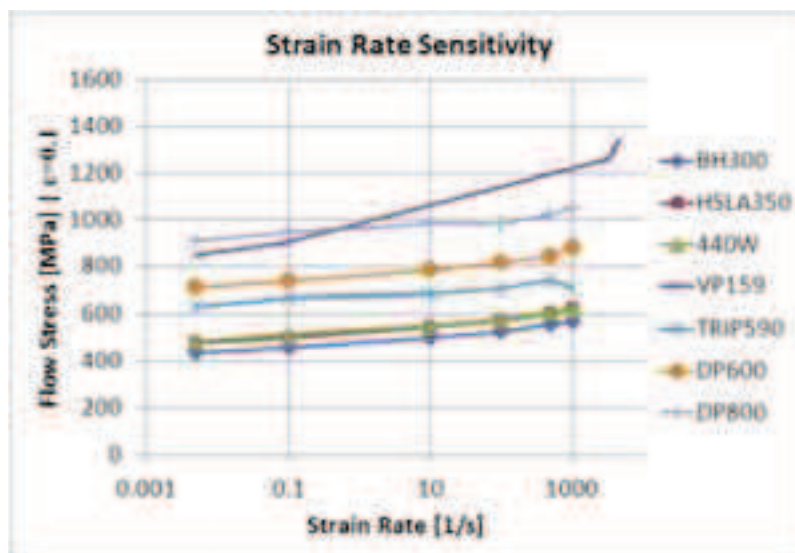
Fig. 2 Strain rate sensitivity of analyzed AHSS
