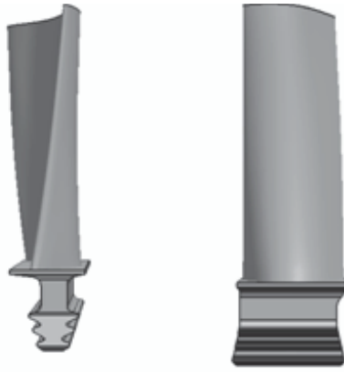
Fig. 1. Complete blade model made in Unigraphics NX 5 program
