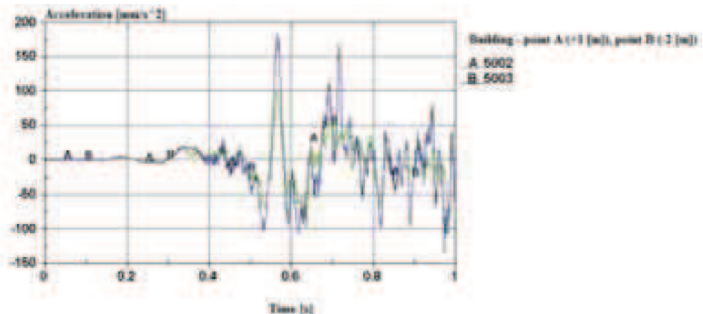
Fig. 7. Amplitude of the vibration acceleration of the foundation of the building in the X direction
