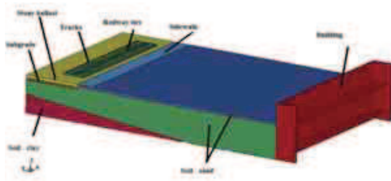
Fig. 6. Diagram of computational model
