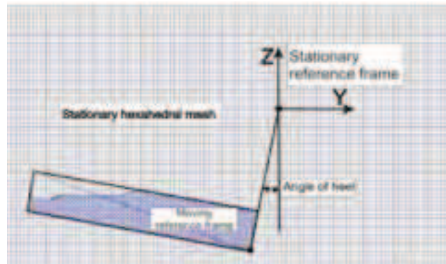
Fig. 6. Computational mesh and two coupled reference frames systems
