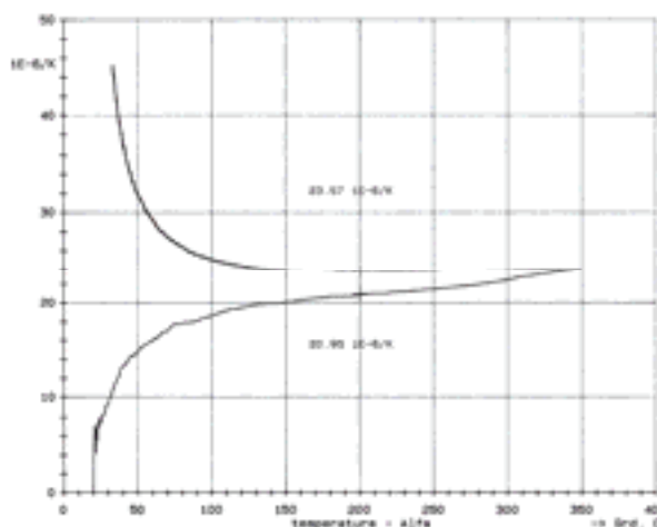
Fig. 2. The course of the coefficient of thermal expansion in the function of the temperature during warming and cooling for standard piston material
