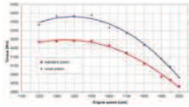
Fig. 10. Courses of maximum torque M [Nm] versus engine rotational speed
