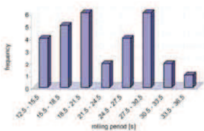
Fig. 4. Histogram of the rolling periods of the ship B-354 in typical loading conditions
