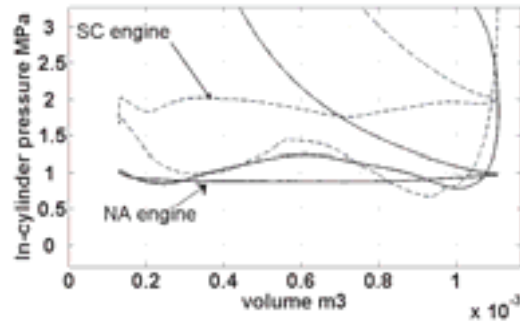
Fig. 3. Charge exchange area in the p-V diagram for the NA and the SC engine
