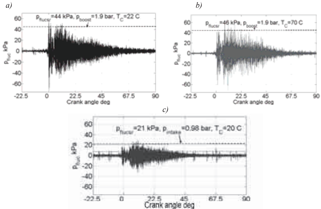
Fig. 6. p_{fluc} for the SC engine (a,b) and the NA engine (c) with the parameters provided in the figures
