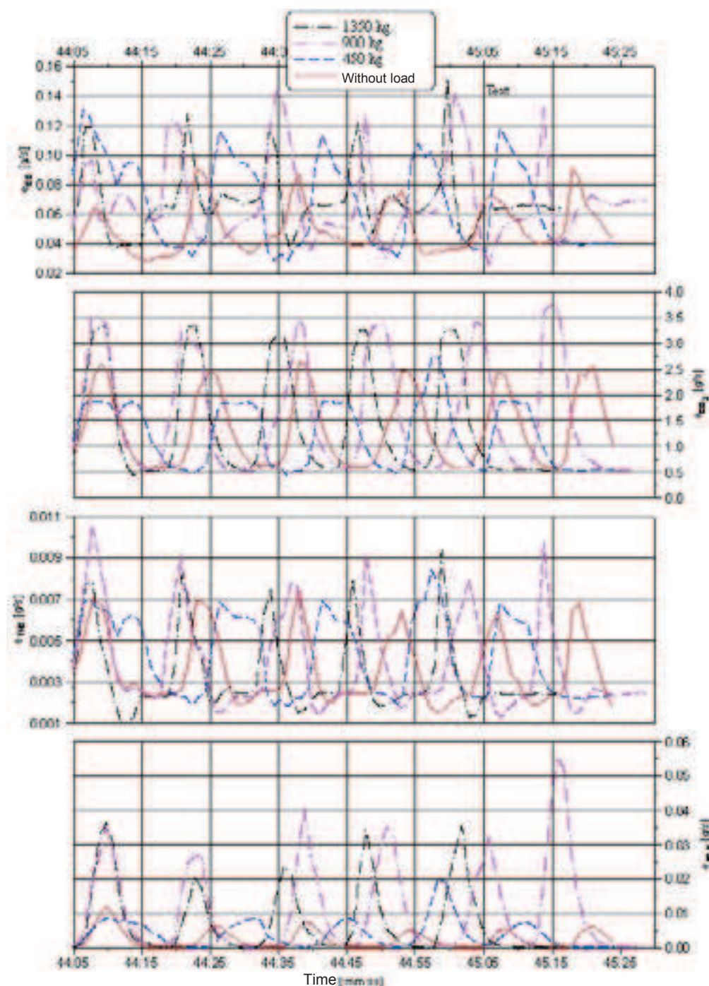
Fig. 2. The course of pollutants emission intensity from a forklift truck during lifting loads of different weights
