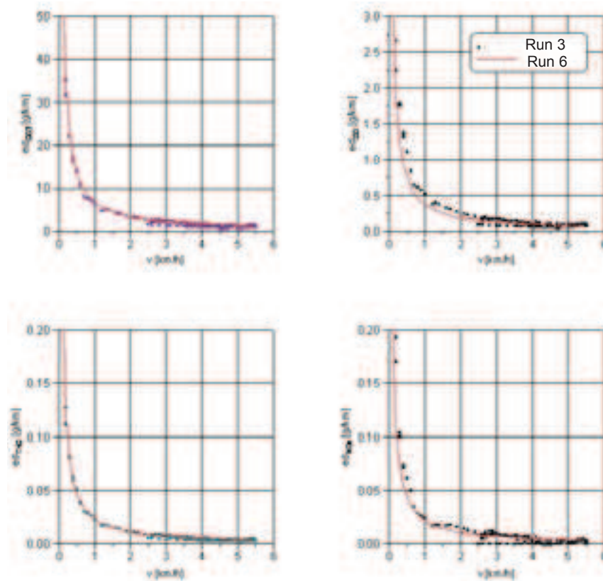
Fig. 5. Change in the road emissions of the selected exhaust components emitted from a forklift truck as a function of speed
