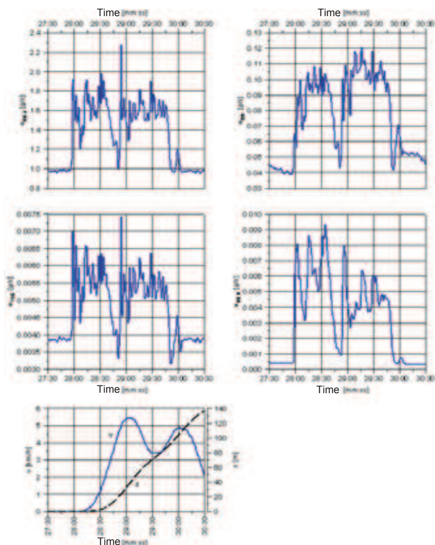
Fig. 4. Change in emission intensity of selected exhaust components emitted from a forklift truck moving during operation; run No. 6
