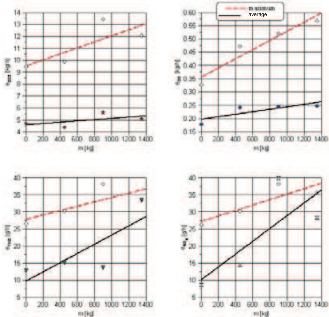
Fig. 3. The course of the emission intensity changes from the forklift H16T-02W as a function of the load lifted
