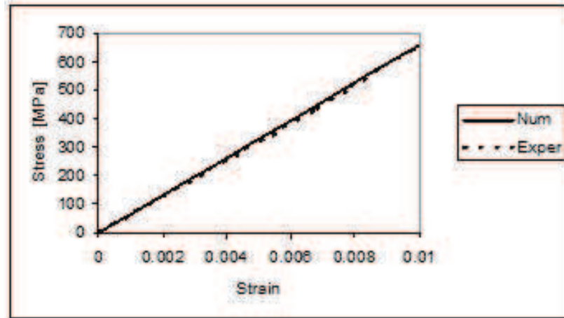
Fig. 5. Comparison of experimental (Exper) and FEM analysis (Num) results
